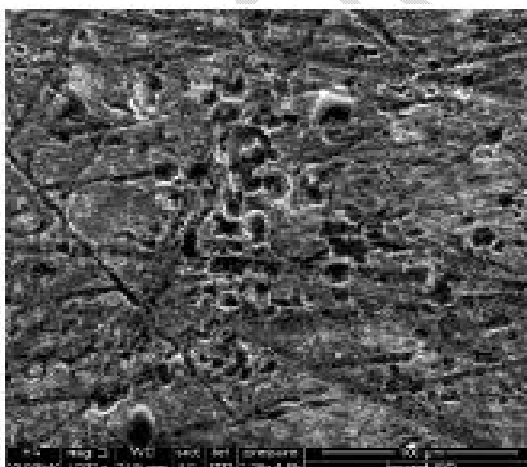
With Ni-complex
