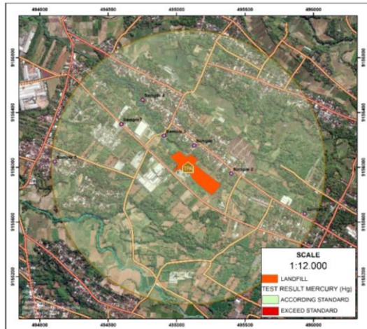
Figure 6. Hg Distribution
