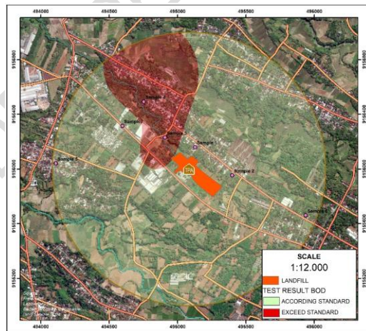
Figure 3. BOD Distribution
