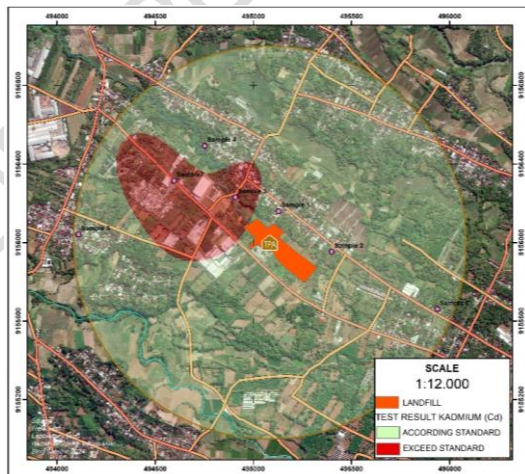
Figure 7. Cd Distribution
