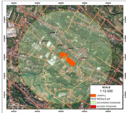
Figure 2. pH Distribution
