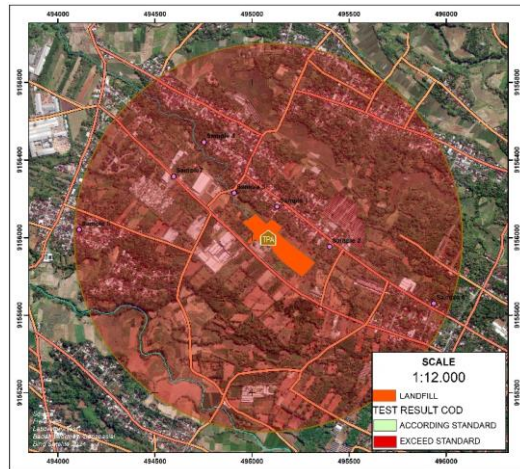
Figure 4. COD Distribution
