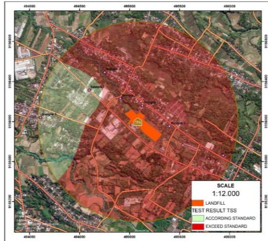
Figure 5. TSS Distribution
