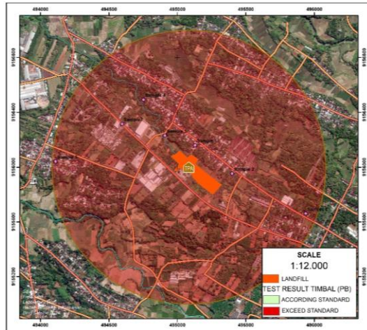
Figure 8. Pb Distribution
