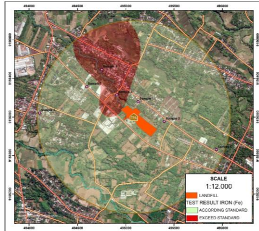
Figure 2. Fe Distribution
