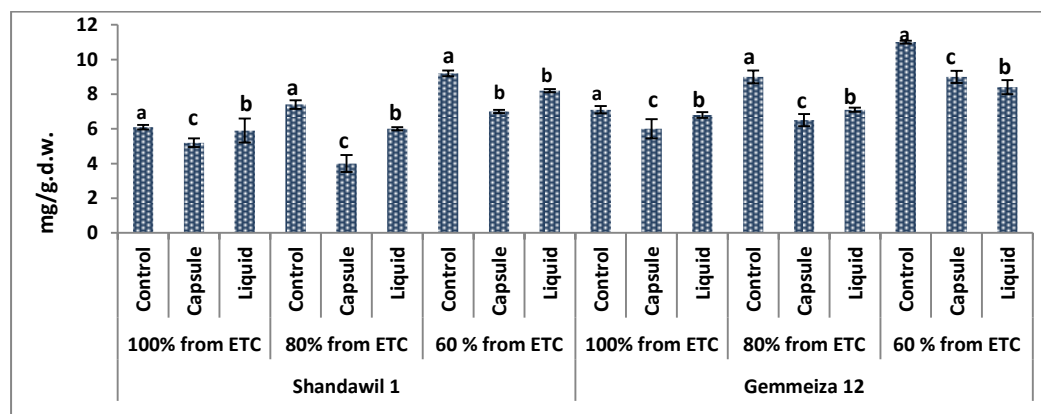
Figure 6. Proline content of two genotype wheat plants Shindawil 1 and Gemmeiza 12 with irrigation intervals 80 and 60 % from ETC treated with either capsules or liquid MSR-M49. Error bars represent the standard deviation between 3 replicates.
