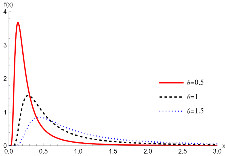
Fig.1. Behavior of the density functions of the IMON distribution.
