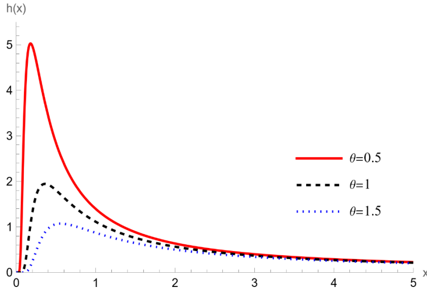
Fig.2 Behavior of the hazard rate function of the IMON distribution.
