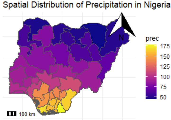
Fig. 1: State average spatial distribution of precipitation in Nigeria
