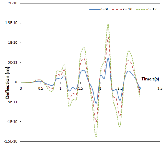
Figure 14: The deflection profile of the moving mass system's fixed-fixed non-uniform damped Rayleigh beam under the influence of a harmonic moving load for different speed values
