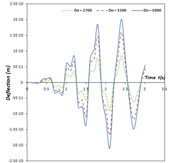
Figure 20: The deflection profile of the moving mass system's fixed-fixed non-uniform damped Rayleigh beam under the influence of a harmonic moving load for different damping coefficient values
