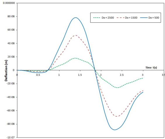
Figure 8: The deflection profile of the moving mass system's pinned-pinned non-uniform damped Rayleigh beam under the influence of a harmonic moving load for different damping coefficient values
