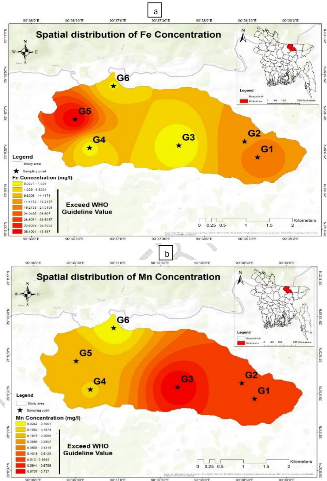
Fig. 3. Spatial distribution of (a) Iron (Fe) and (b) Manganese (Mn) concentration
