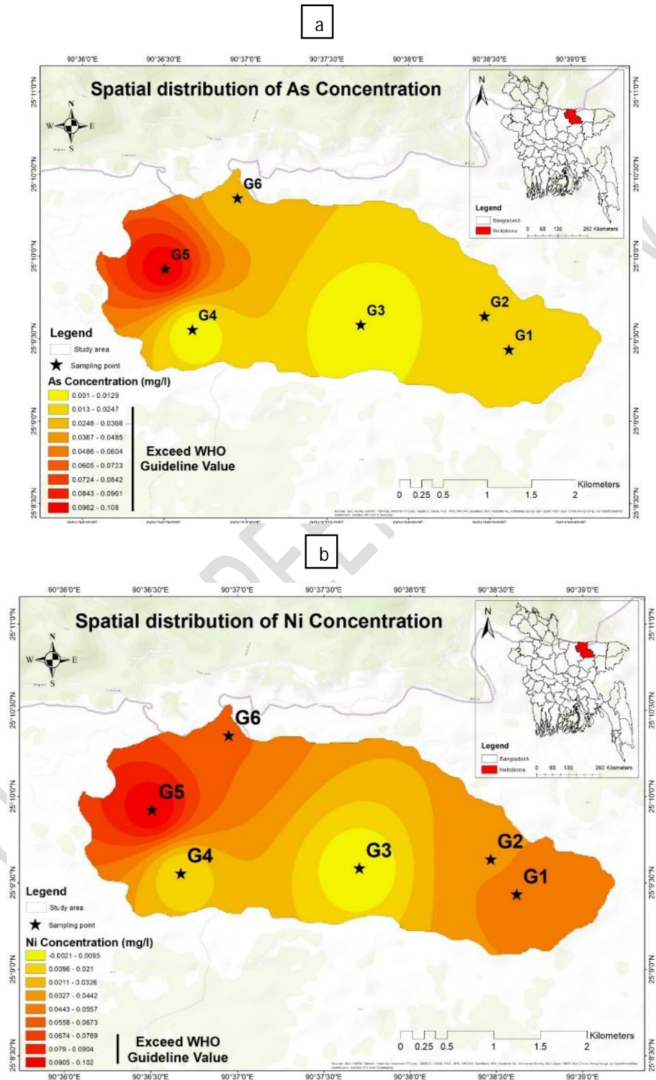
Fig. 2. Spatial distribution of (a) Arsenic (As) and (b) Nickel (Ni) concentration
