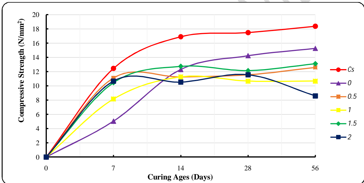
Figure 5: Compressive Strength of Wood Ash Blended Cement Concrete.
