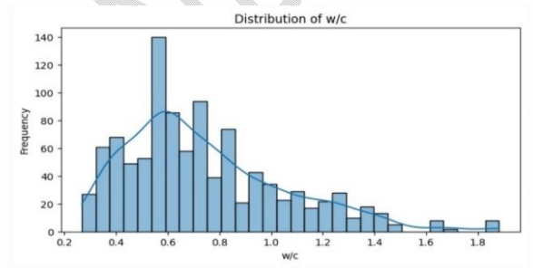
Figure 7: Distribution plots for each parameter.
