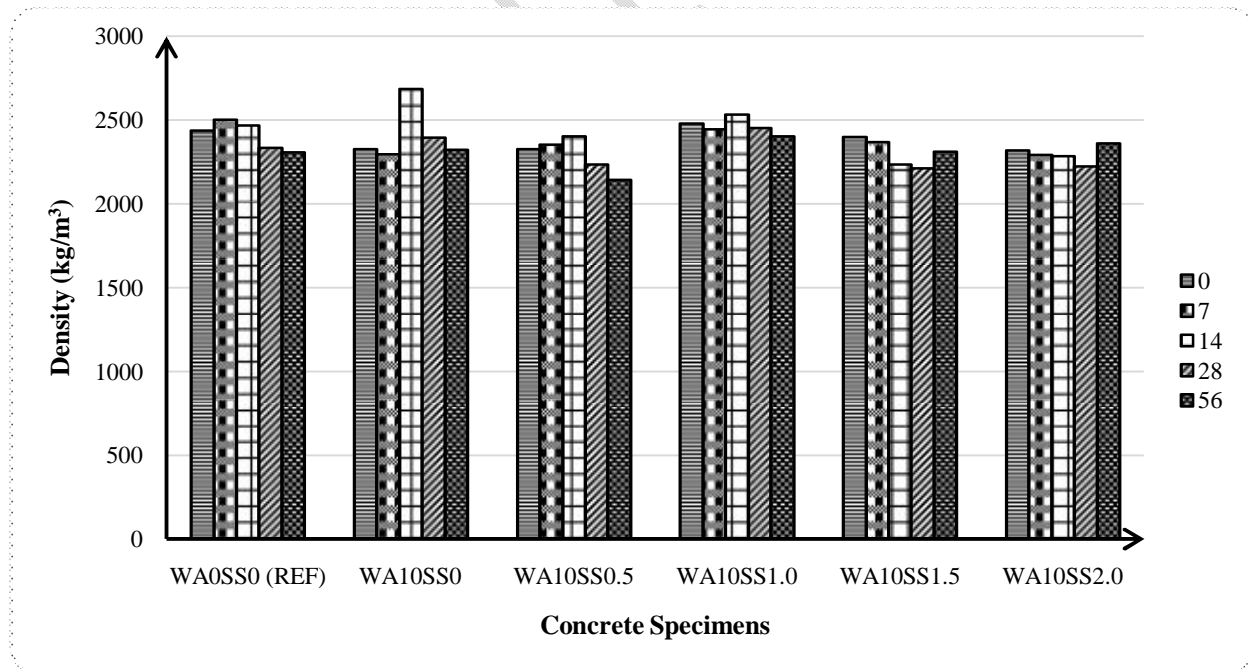
Figure 4: Density of Wood Ash Blended Cement Concrete.
