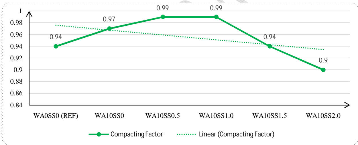
Figure3: Compacting Factor of Wood Ash Blended Cement Concrete.
