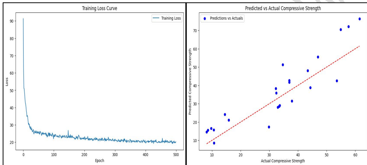
Figure 8: Training Loss per epoch curve. Figure 9: Predicted vs Actual Compressive Strength.
