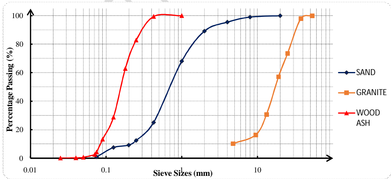
Figure 1: Particle Size Distribution Curve.
