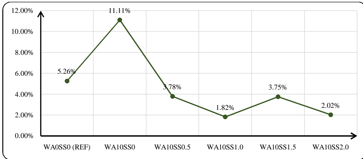
Figure 6: Water Absorption of Wood Ash Blended Cement Concrete.
