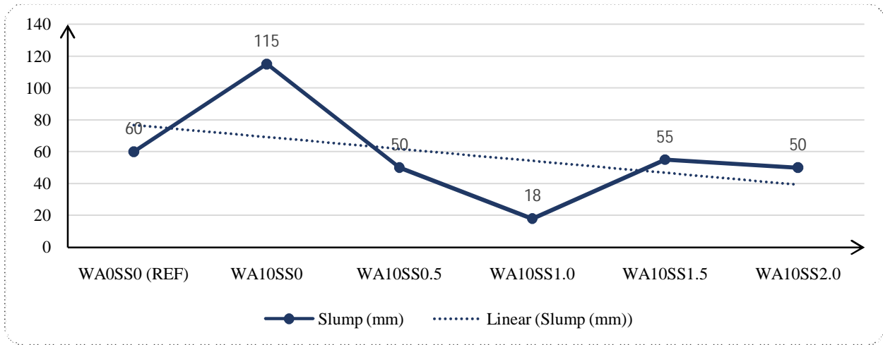
Figure2: Slump Test of Wood Ash Blended Cement Concrete.
