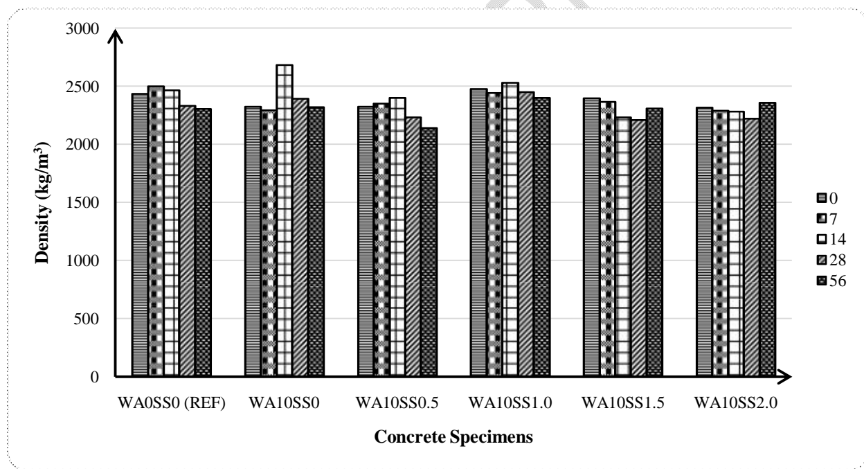
Figure 4: Density of Wood Ash Blended Cement Concrete.
