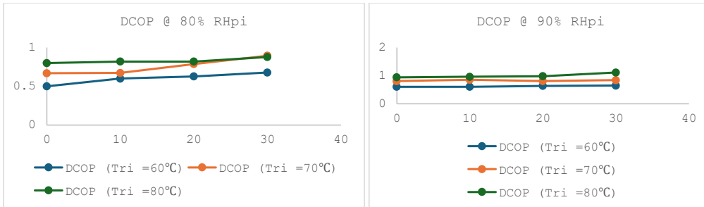
Fig.8. DCOP at 60%, 70%, 80% and 90% relative humidity of inlet process air.
