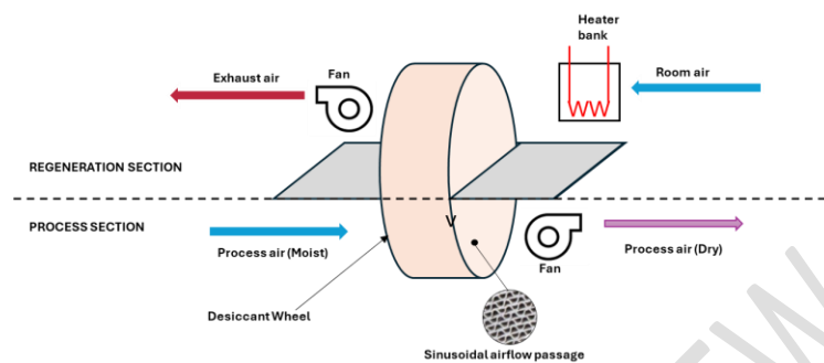
Fig.2. Schematic diagram of desiccant dehumidifier system.
