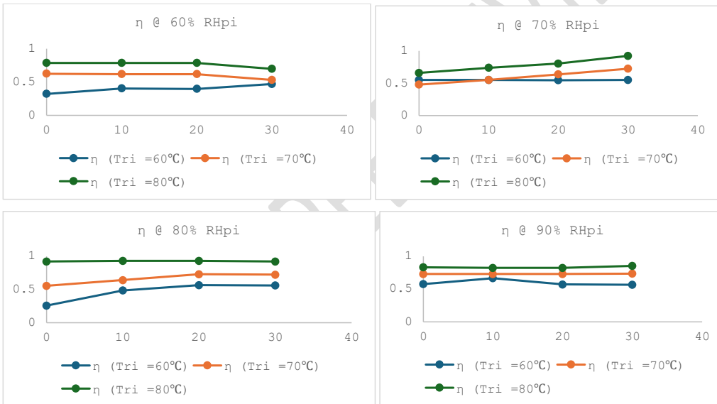
Fig.6. Dehumidification effectiveness at different relative humidity (60%, 70%, 80% and 90%) of process air.
