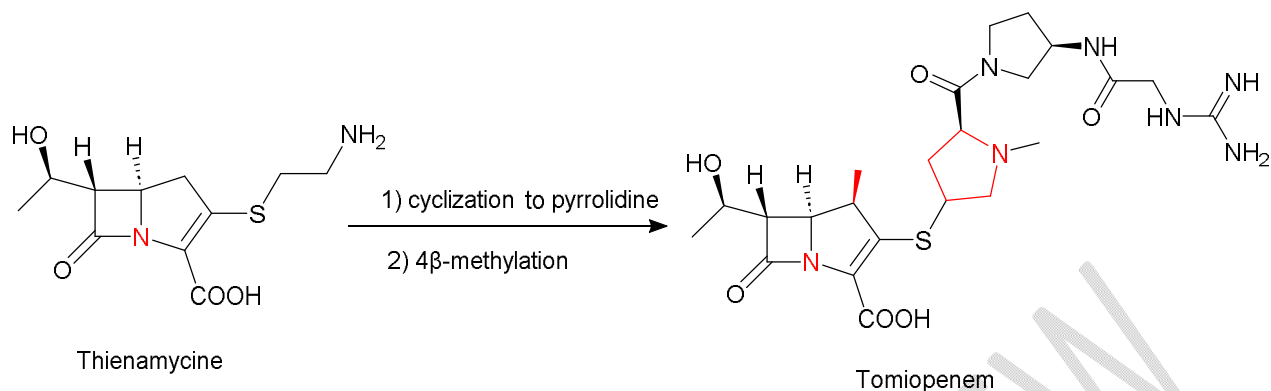
Figure 13: Chemical structure of Tomiopenem
