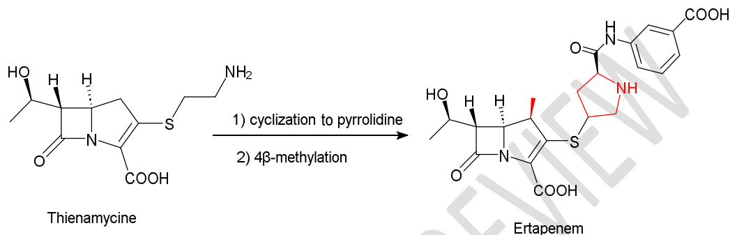
Figure 11: Chemical structure of Ertapenem
