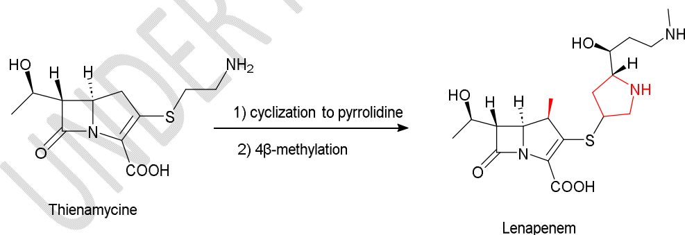
Figure 12: Chemical structure of Lenapenem
