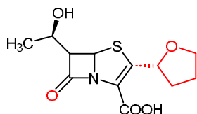
Figure 18 : Chemical structure of Faropenem
