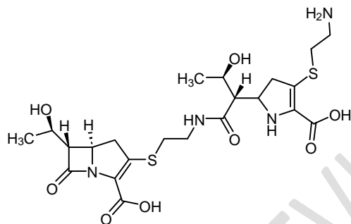
Figure 3: Chemical structure of a thienamycin dimer
