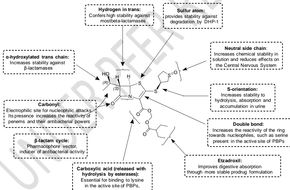
Figure 17: Diagram of structure-activity relationships around of Sulopenem[74]
