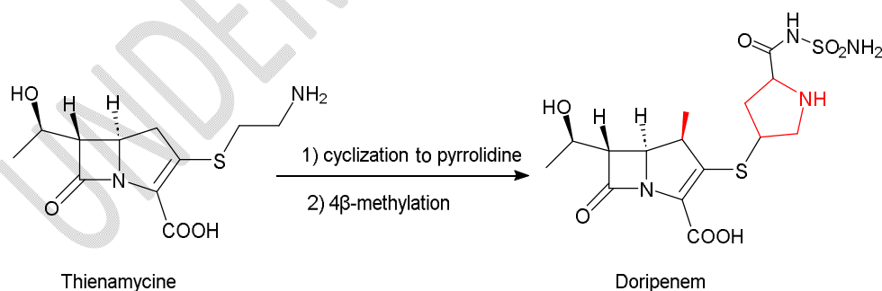
Figure 10: Chemical structure of Doripenem
