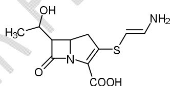
Figure 1: Chemical structure of olivanic acid
