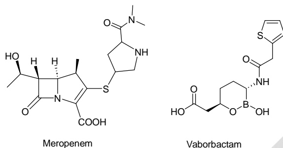
Figure 21: Meropenem–vaborbactam combination
