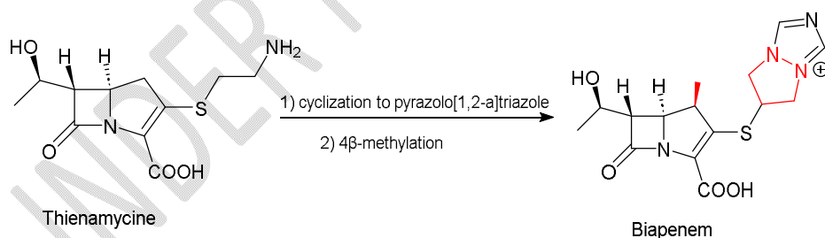
Figure 14: Chemical structure of Biapenem
