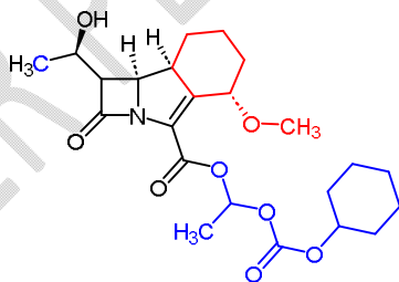
Figure 19: Chemical structure of Sanfetrinem-Cilexetil
