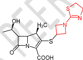
Figure 15: Chemical structure of Tebipenem
