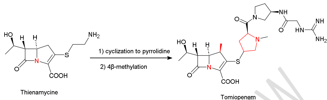
Figure 13: Chemical structure of Tomopenem
