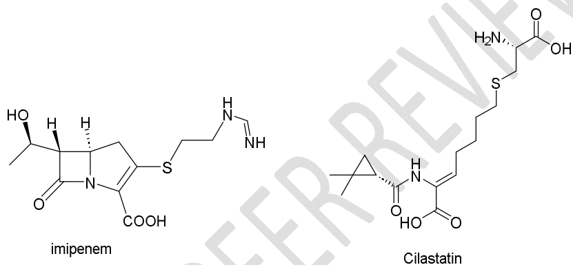
Figure 6: Chemical Structure of Imipenem-Cilastatin
