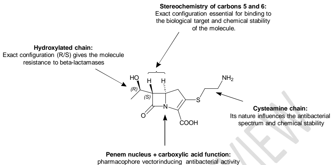
Figure 4: Structural elements essential for maintaining antibacterial activity.
