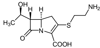
Figure 2: Chemical Structure of Thienamycin
