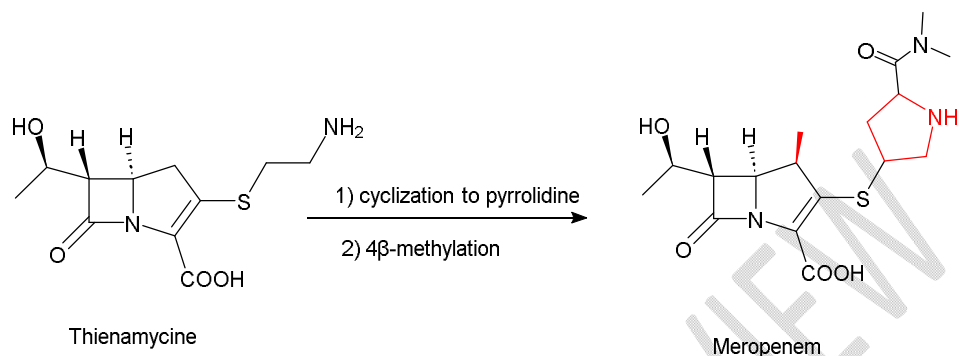
Figure 9: Chemical structure of Meropenem
