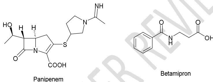
Figure 8: Chemical structure of Panipenem/Betamipron
