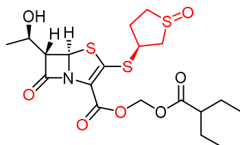
Figure 16: Chemical Structure of Sulopenem-Etzadroxil
