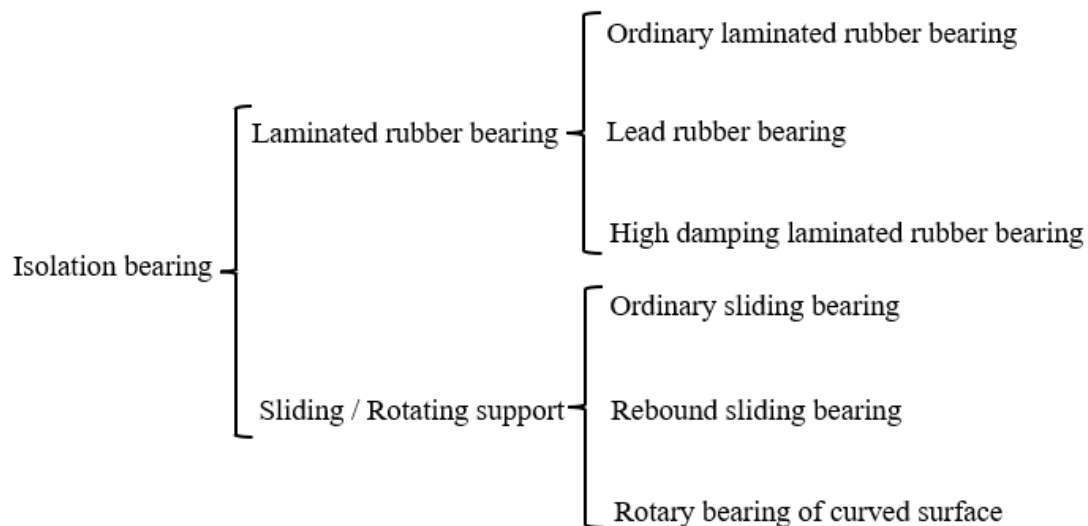
Fig.1 Type of isolation bearing
