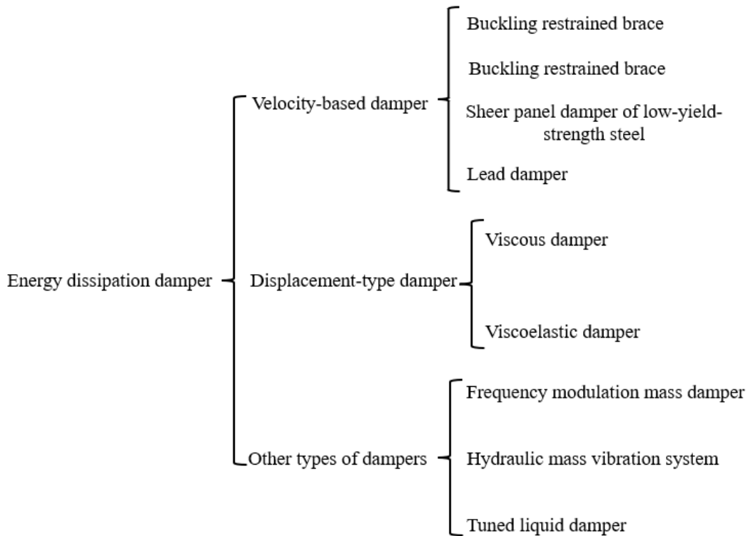
Fig.3 Classification of energy dissipation shock absorbers
