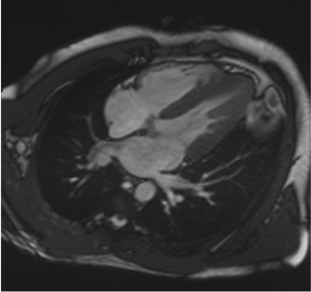
FIGURE 2. CARDIAC MRI WITHOUT ABNORMALITIES
