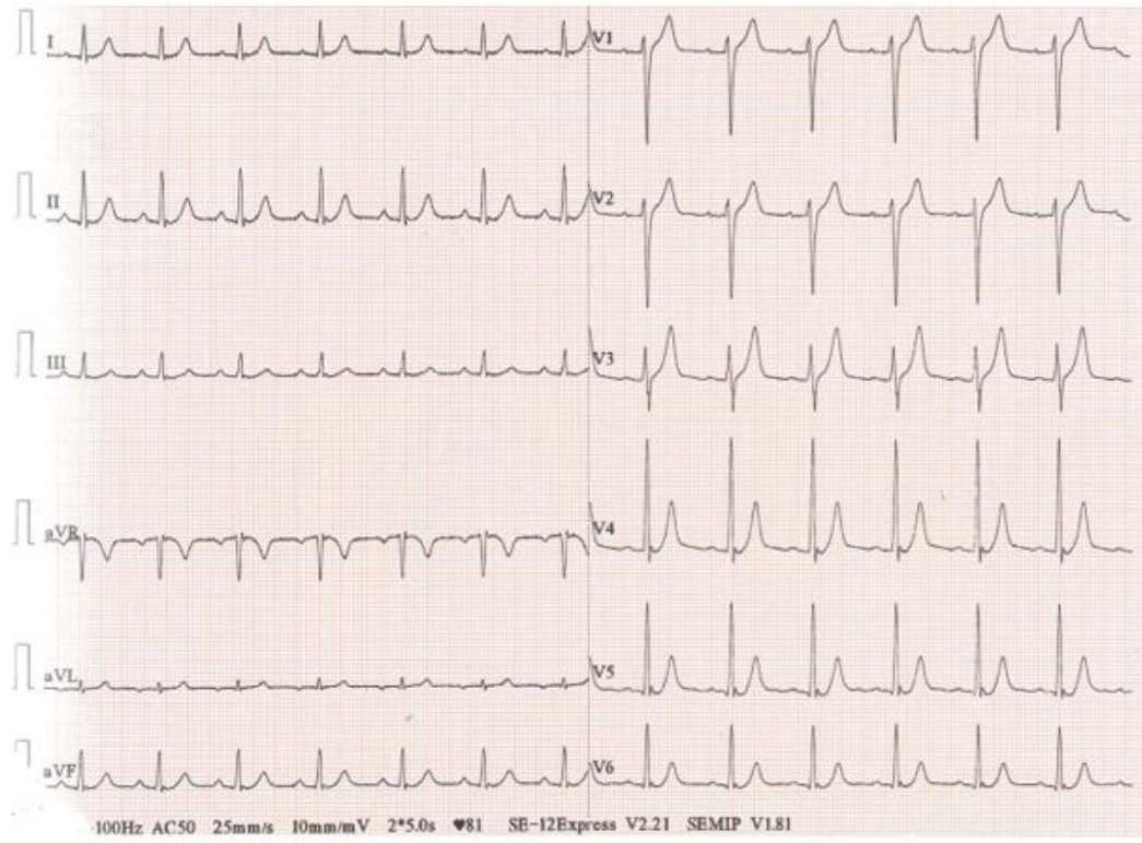
FIGURE 4. POST CRITICAL ECG SHOWING EARLY REPOLARIZATION WITH A CLEAR REGRESSION OF ST SEGMENT ELEVATION
