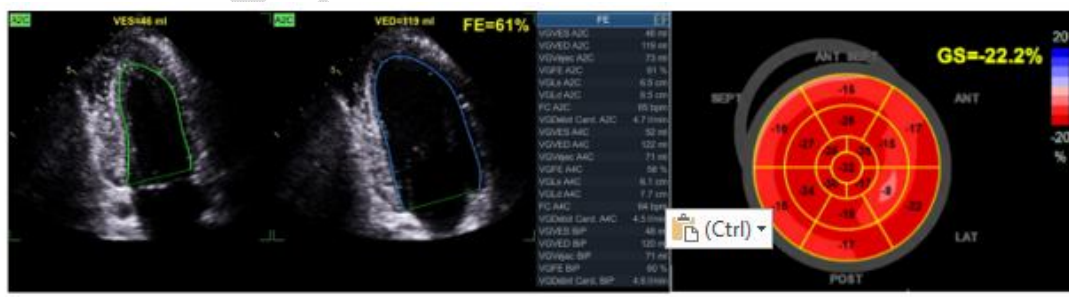
FIGURE 5. NORMALIZATION OF THE EJECTION FRACTION AND THE STRAIN GLOBAL LONGITUDINAL AT THE 1 MONTH FOLLOW UP
