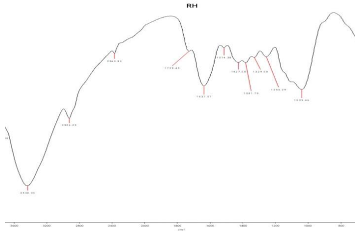
Figure 23. FTIR spectrum of the rice husk sorbent
