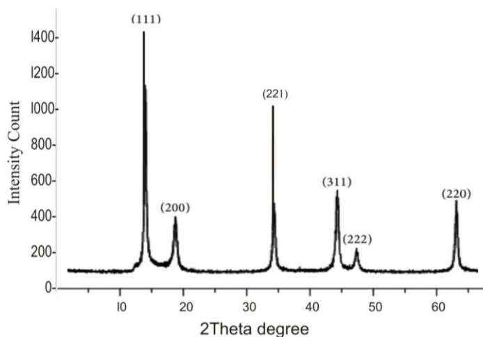
Figure 67. XRD (X-ray Diffraction) spectrum for rice husk nano sorbent
