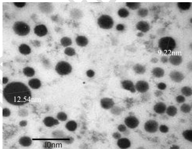
Figure 45. Transmission Electron Microscopy (TEM) of the rice husk sorbent
