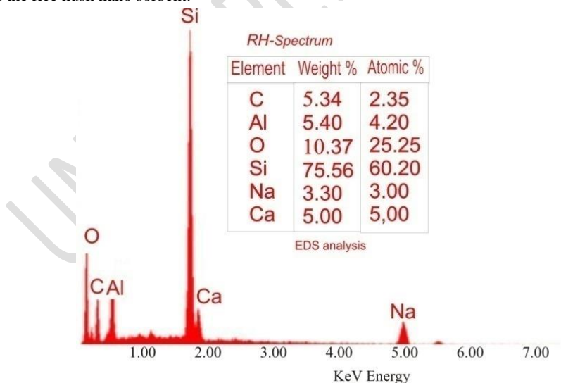
Figure 56. EDX (Energy Dispersive X-ray Spectroscopy) of rice husk nano sorbent
