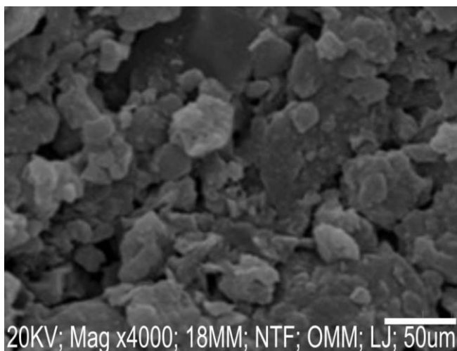
Figure 34. Scanning Electron Micrograph (SEM) of the rice husk sorbent
