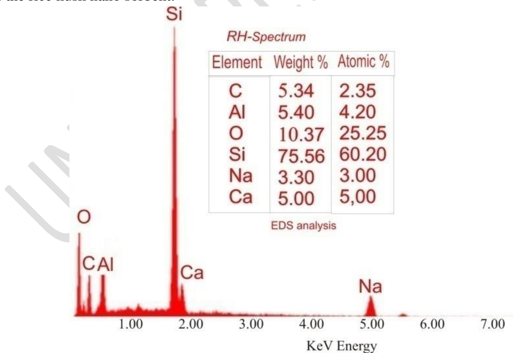
Figure 6. EDX (Energy Dispersive X-ray Spectroscopy) of rice husk nano sorbent
