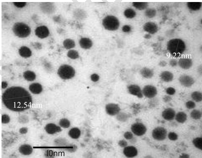
Figure 5. Transmission Electron Microscopy (TEM) of the rice husk sorbent
