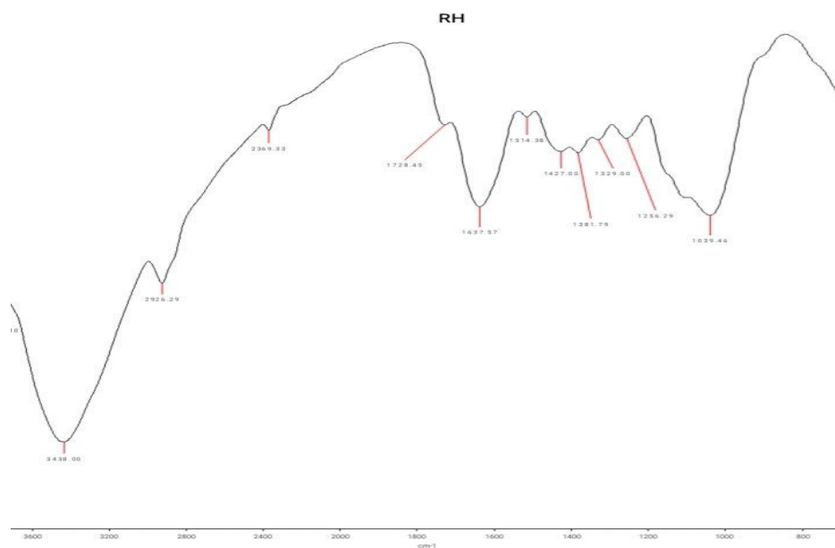
Figure 3. FTIR spectrum of the rice husk sorbent
