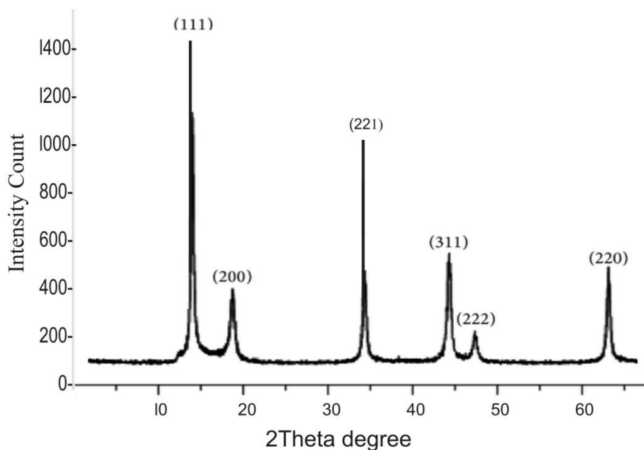
Figure 7. XRD (X-ray Diffraction) spectrum for rice husk nano sorbent
