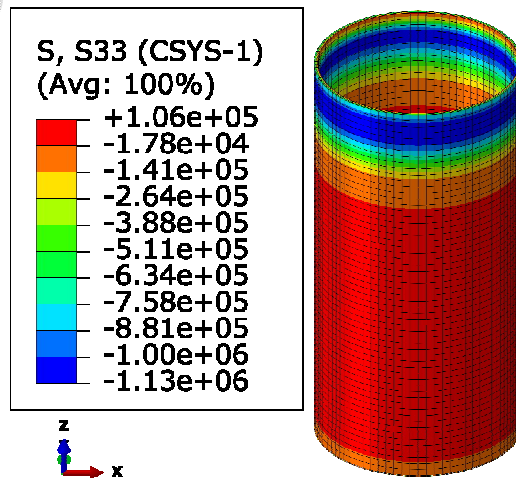
(c)Vertical stress
