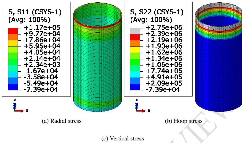
Fig.7 Stress of concrete cylinder under temperature decrease (unit: Pa)
