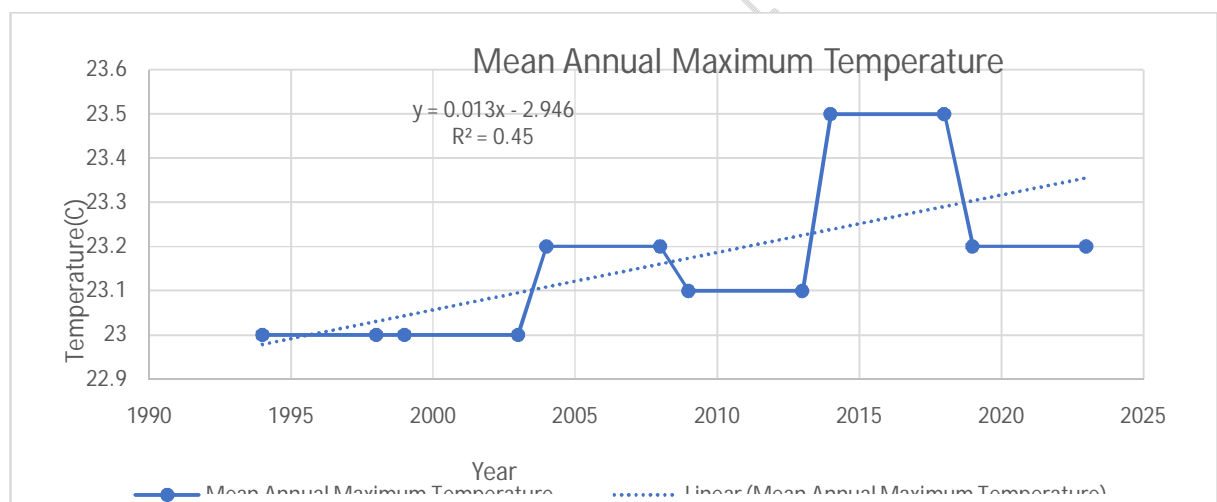
Figure 3: Temperature trends In Meatu District From 1994-2023
