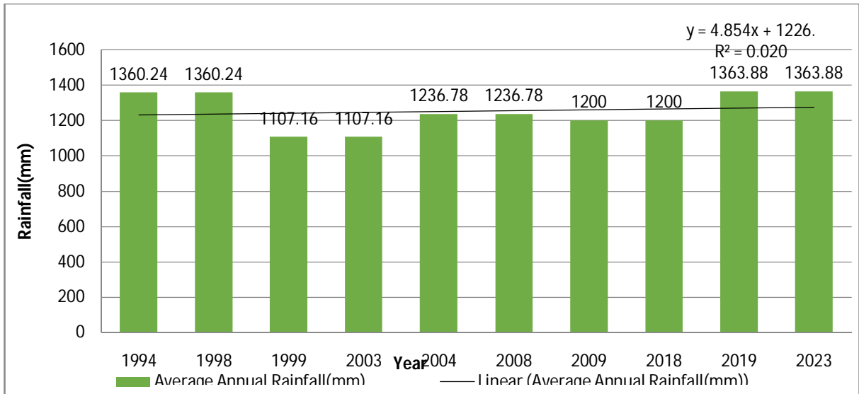
Figure 2: Precipitations of Rainfall Patterns in Meatu District From 1994-2023
