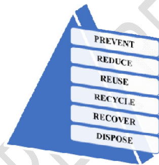
FIGURE 2-Waste management hierarchy
