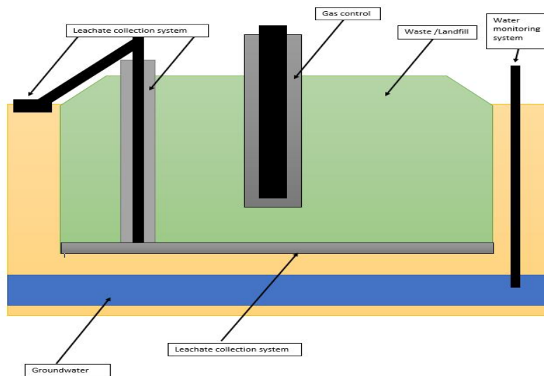
FIGURE 3- Gas collection system (Dada&Mbohwa, 2017).
