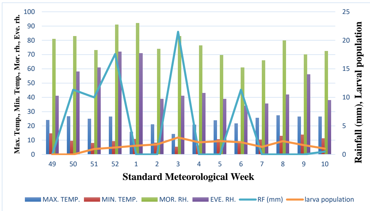
Figure 1: Seasonal incidence of Pod borer, Helicoverpa armigera L. in Chickpea during Rabi season 2023-2024.
