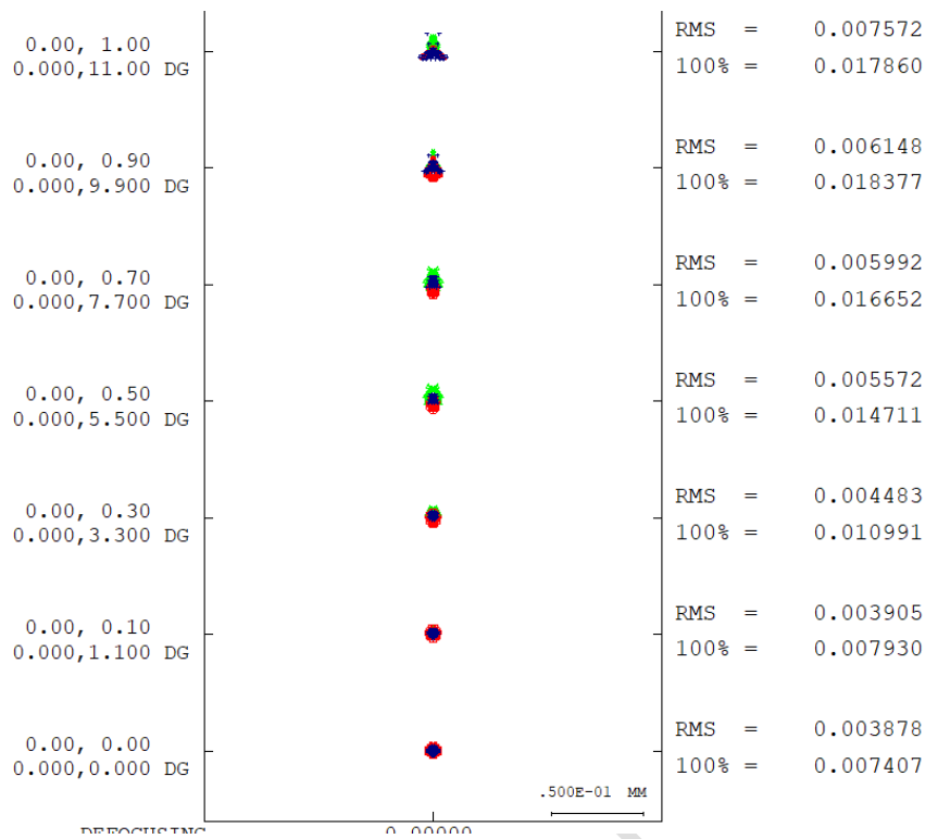
Figure 6 Point diagram of the optical system
