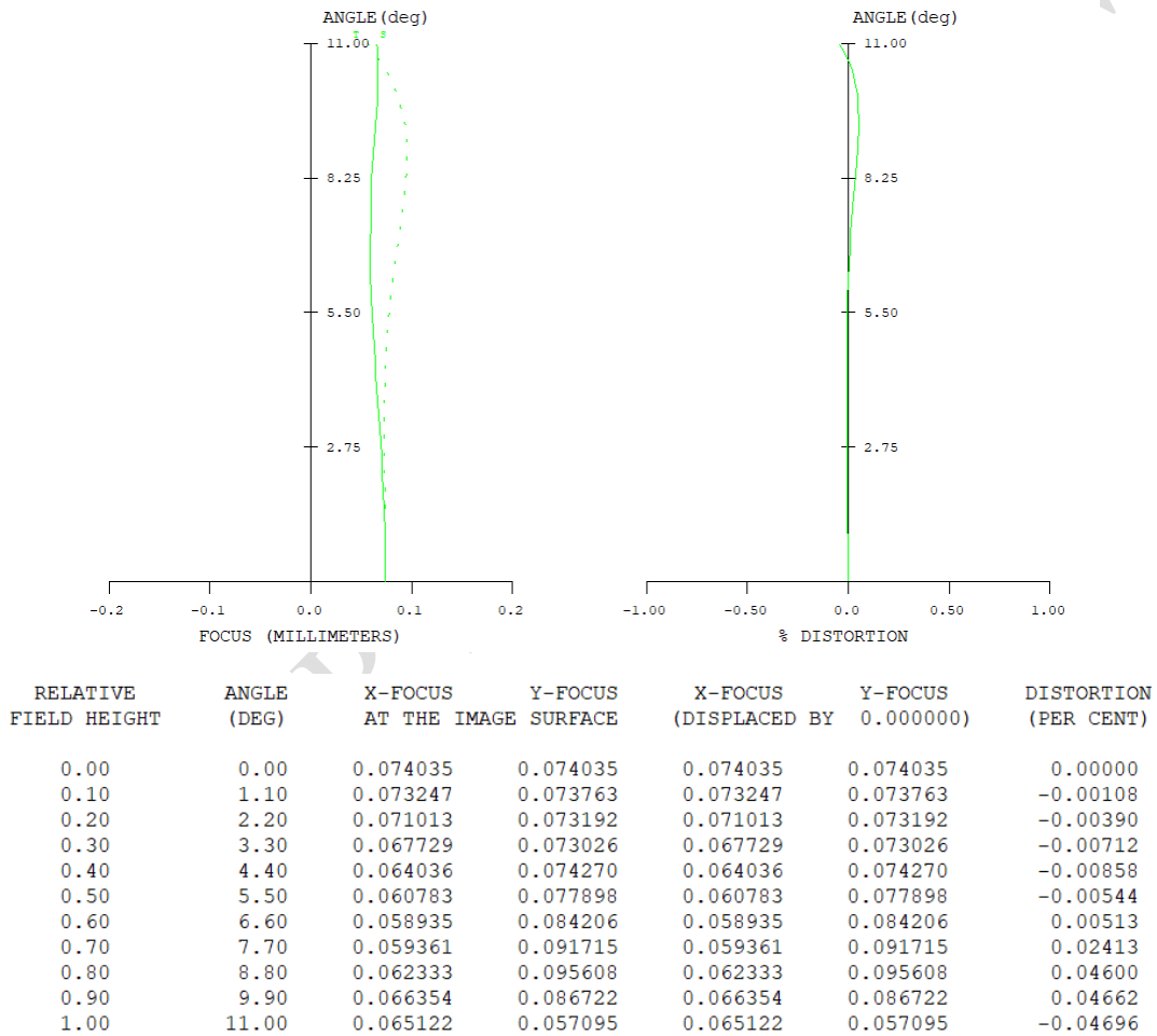
Figure 7 Field curvature and distortion
