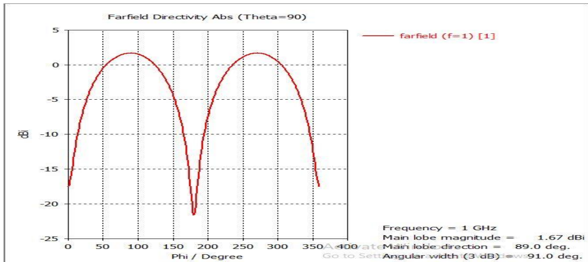
FIG. 1.7 2-D Radiation Pattern of Broadband Microstrip Antenna
