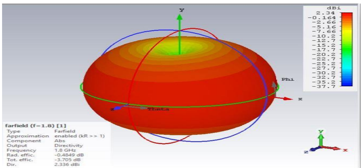
FIG. 1.6 3-D Far field radiation pattern
