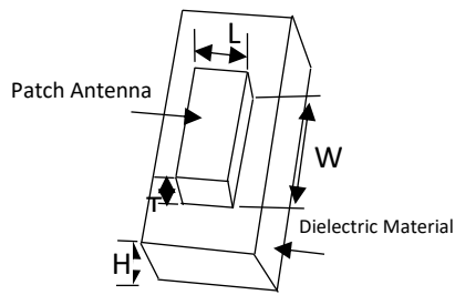
FIGURE 1 simple structure
