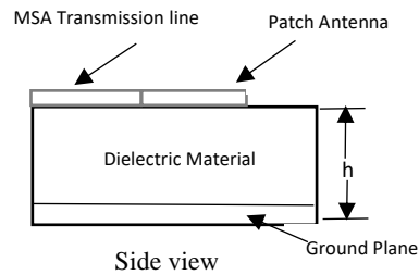
FIGURE 2 Side View
