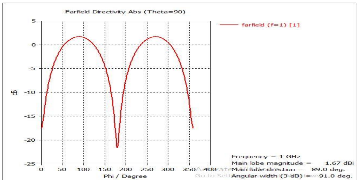
FIGURE 7 2-D Radiation Pattern of Broadband Microstrip Antenna
