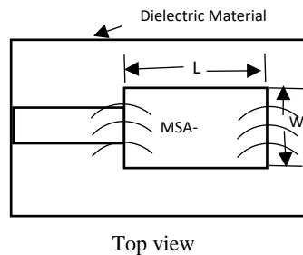
FIGURE 3 Top View
