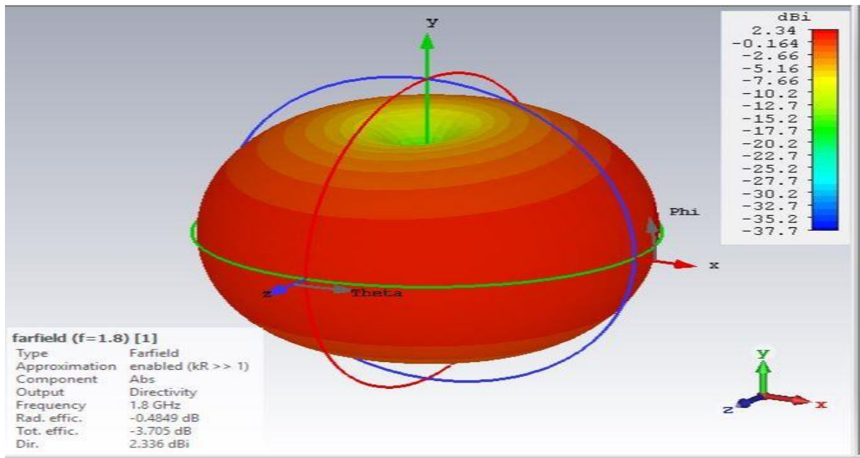
FIGURE 6 3-D Far field radiation pattern
