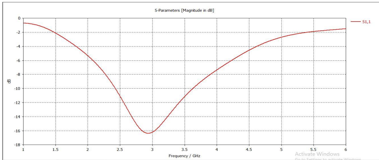
FIGURE 5 S-Parameter
