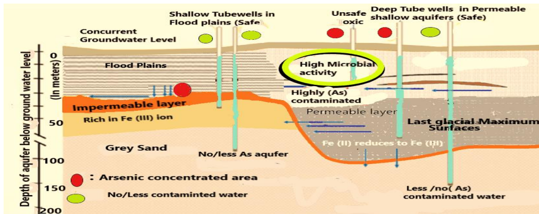
Figure 5: The vertical sections of arsenic invasive areas in the Ganga-Bhagirath River system (Source modified Majumdar et al., 2011):
