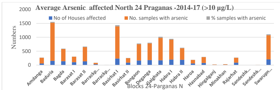
Fig 10 (f): The highly arsenic-contaminated N-24 Parganas District of West Bengal; 2014-17
