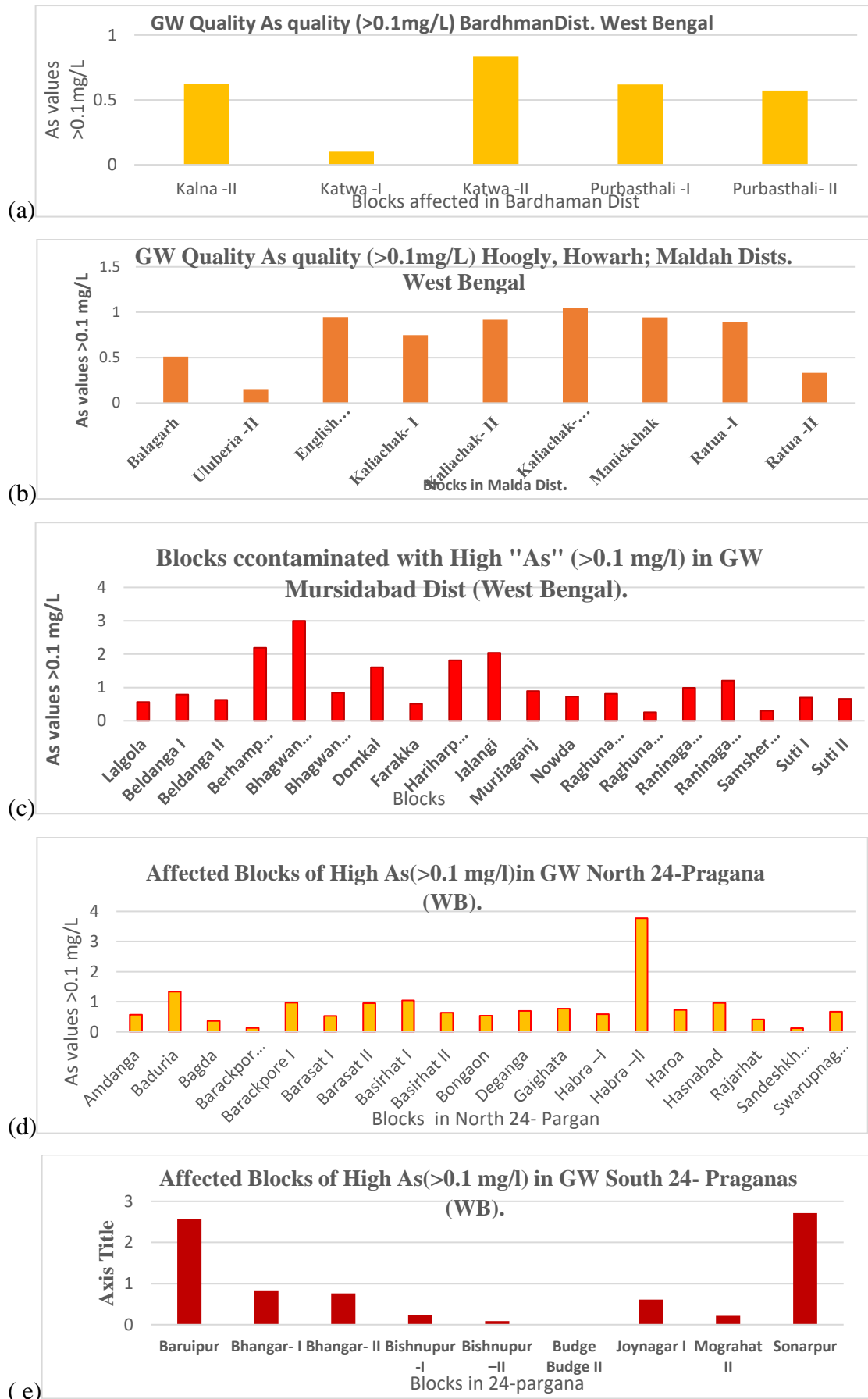
Fig 9 (a-e): The Arsenic contaminated districts of West Bengal in India (Source CGWB -2016)
