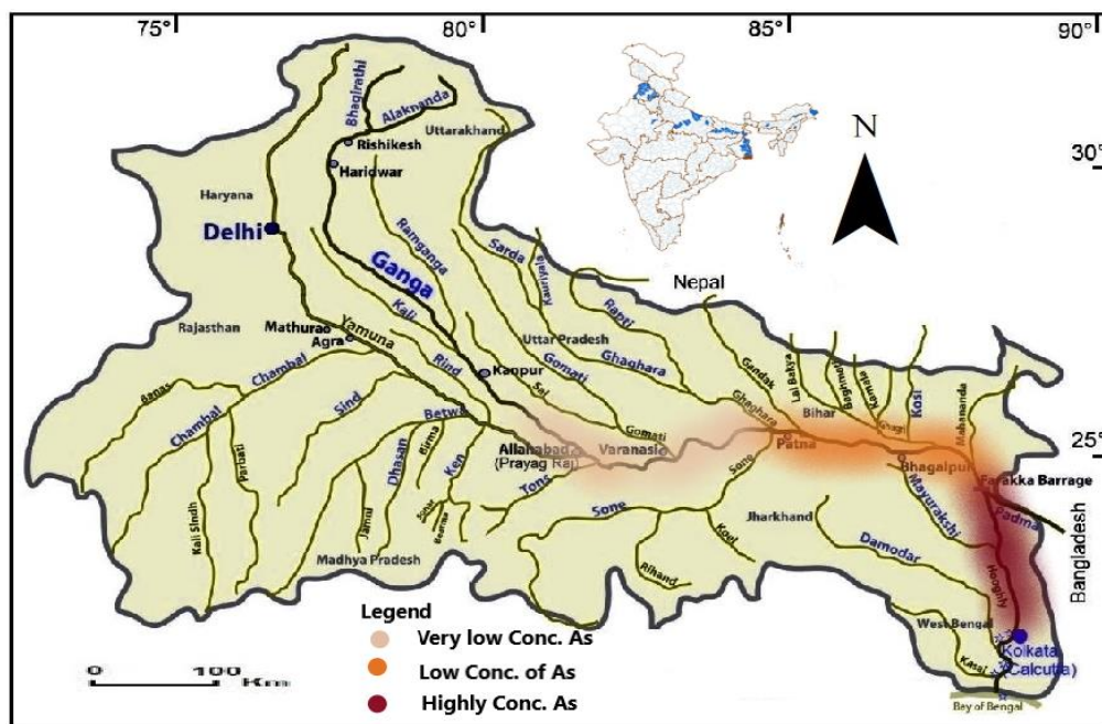
Figure 7: The Arsenic toxicity in India from Siwalik Range to BoB in South 24 Parganas
