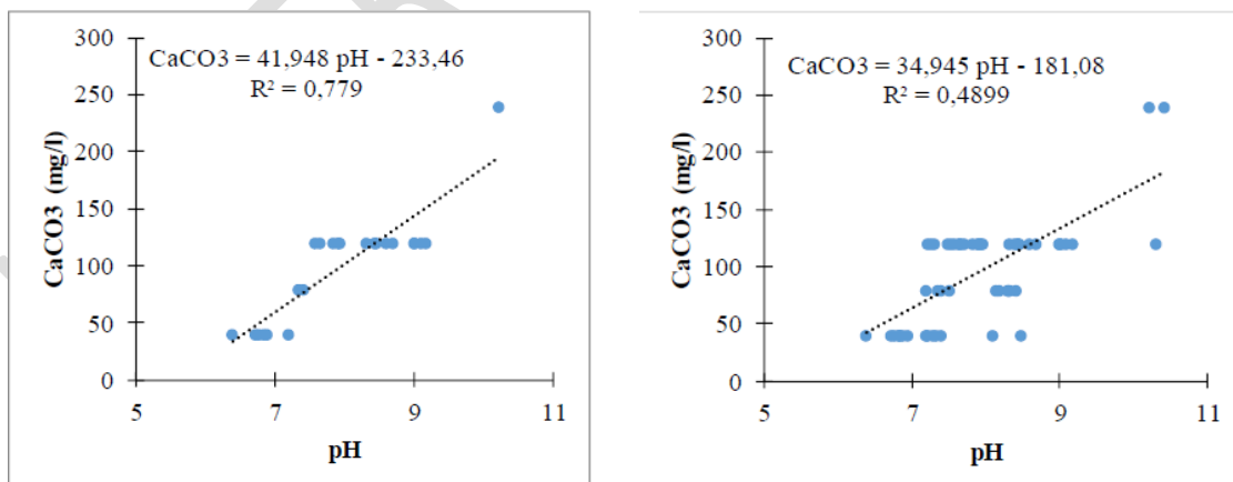
Figure 1: pH-alkalinity relationship for (a) the artificial method and (b) the semi-natural method.
