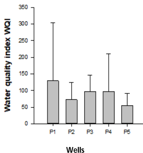
Fig.3. Spatial variation of water quality index (WQI)
