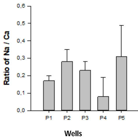
Fig.4. Sapatial variation of the ratio Na/Ca
