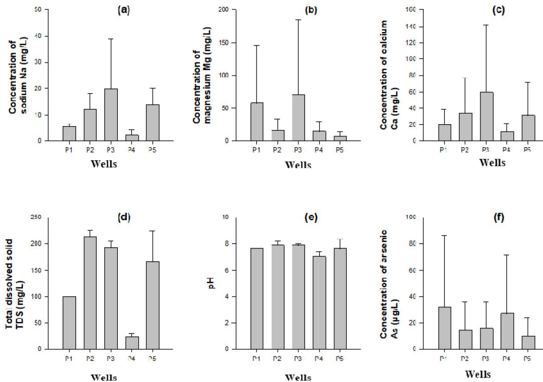
Fig. 2. Spatial variations of sodium (a), magnesium (b), calcium (c), total dissolved solids (d) and arsenic (f) concentrations, and spatial variations of pH (e),
