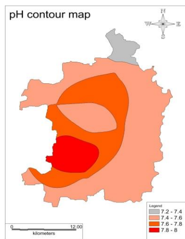
Fig. 2 – Spatial Distribution of pH
