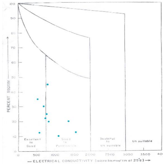
Fig. 7: H. Wilcox's Diagram
