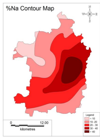
Fig. 6: Spatial distribution of %Na
