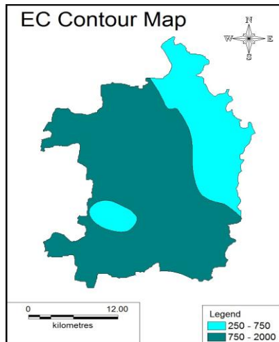
Fig. 3 – Spatial Distribution of EC
