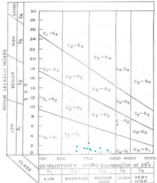
Fig. 5: US Salinity Diagram
