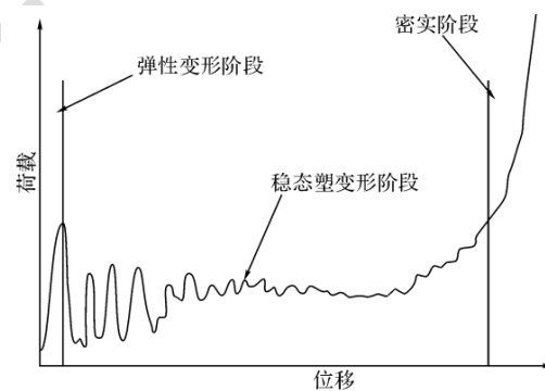
Fig. 5 Load-displacement curves of a typical elasto-plastic honeycomb structure under anisotropic compressive loading [12]
