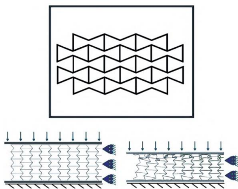
Fig. 4 Negative Poisson's ratio concave hexagonal honeycomb structure [11]
