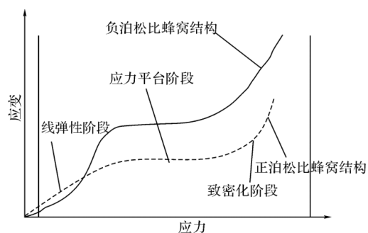
Fig. 6 Stress-strain curve of honeycomb structure [13]
