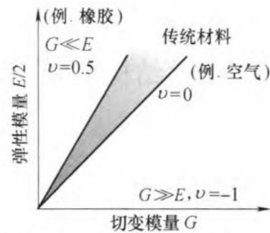
Fig. 2 Relationship between shear modulus G , modulus of elasticity E , and Poisson's ratio \nu of the material
