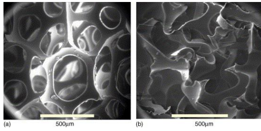
Fig. 7 Scanning electron micrographs of normal polymer foam (left) and negative Poisson's ratio polymer foam (right) [35]
