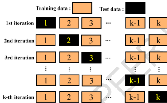
Fig. 3. K-fold cross-validation.
