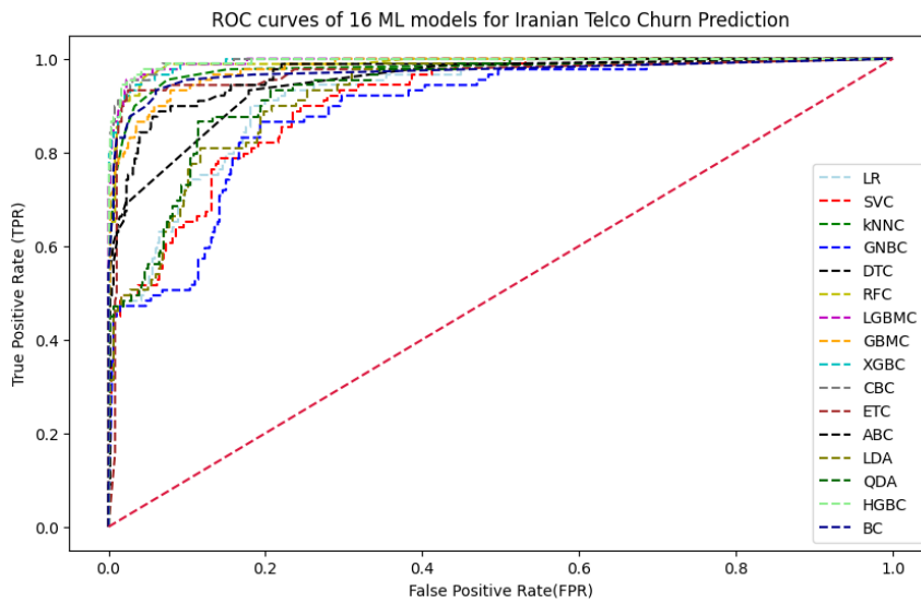
Fig. 5. ROC curves of 16 ML Models with Iranian Telco Customer Churn Prediction.
