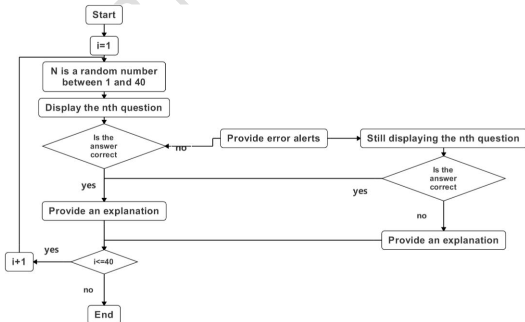
Figure 2: Use of linked lists in Scratch - Random question generation process diagram
