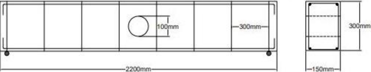
Fig. 3(b). Illustration of test beams (B3 and B5) with opening and 100mm diameter PVC pipe placed transversely at midspan.
