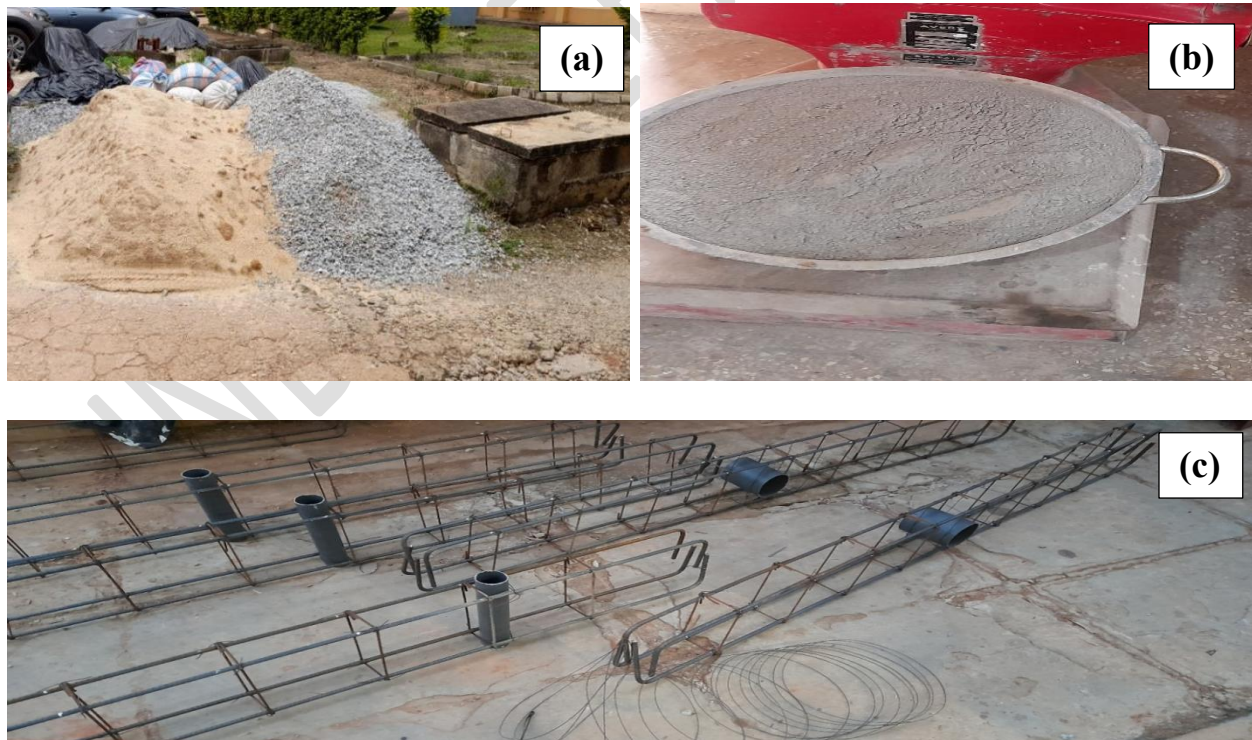
Fig. 1. Materials: (a) sand and gravel, (b) cement, (c) 12mm steel rebars with 8mm stirrups and PVC pipes.
