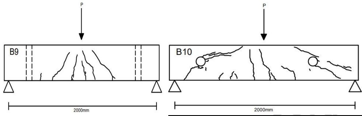
Fig. 7. Illustration of crack patterns on test and control beams
