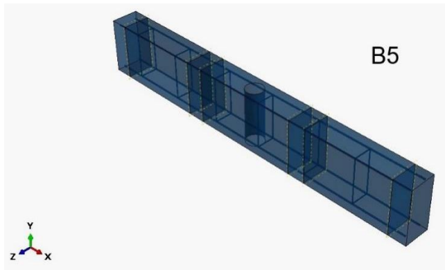
Fig. 3(f). Illustration of test beams modelled using ABAQUS software.
