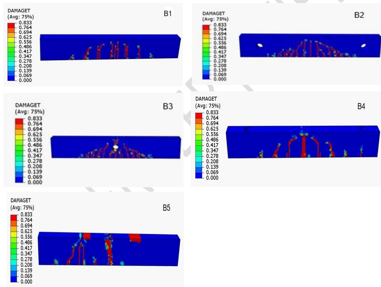
Fig. 9. Crack patterns
