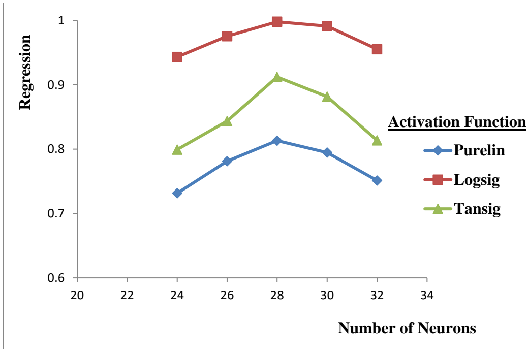
Figure 1: The Effect of Number of Neuron on Regression Value at Different Activation Function
