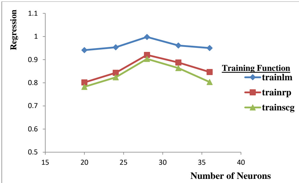
Figure 3: The Effect of Number of Neuron on Regression Value at Different Training Functions
