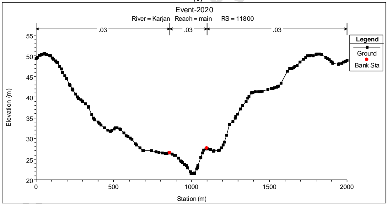
Fig 6 Station-elevation data of extracted cross-sections in HEC-RAS geometric data editor window
