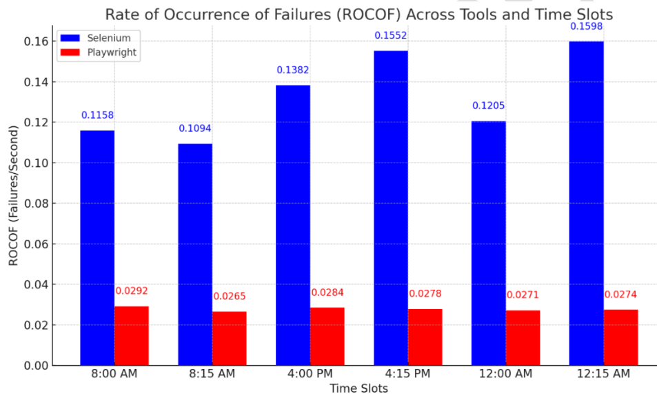
Figure 1 Bar chart represents the ROCOF for Selenium and Playwright t across various time slots
