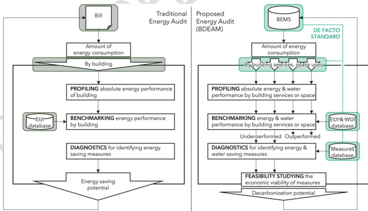
Fig. 4. Conventional (left) and proposed (right) energy audit frameworks.
