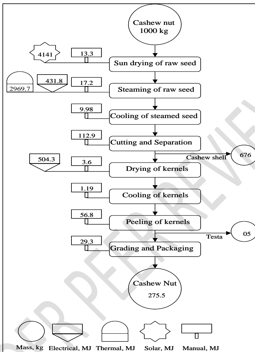
Fig.3 Representative process flow diagram with symbols for energie
