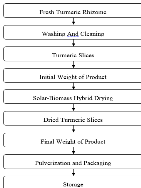
Fig. 1 Process flow chart of turmeric slices drying
