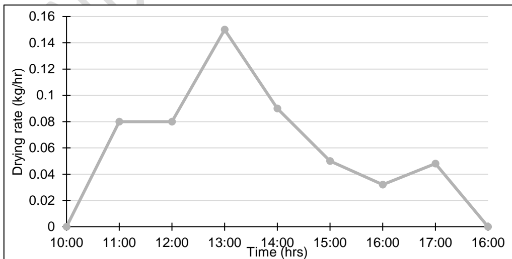
Fig. 2. Drying rate of turmeric slices during full load test
