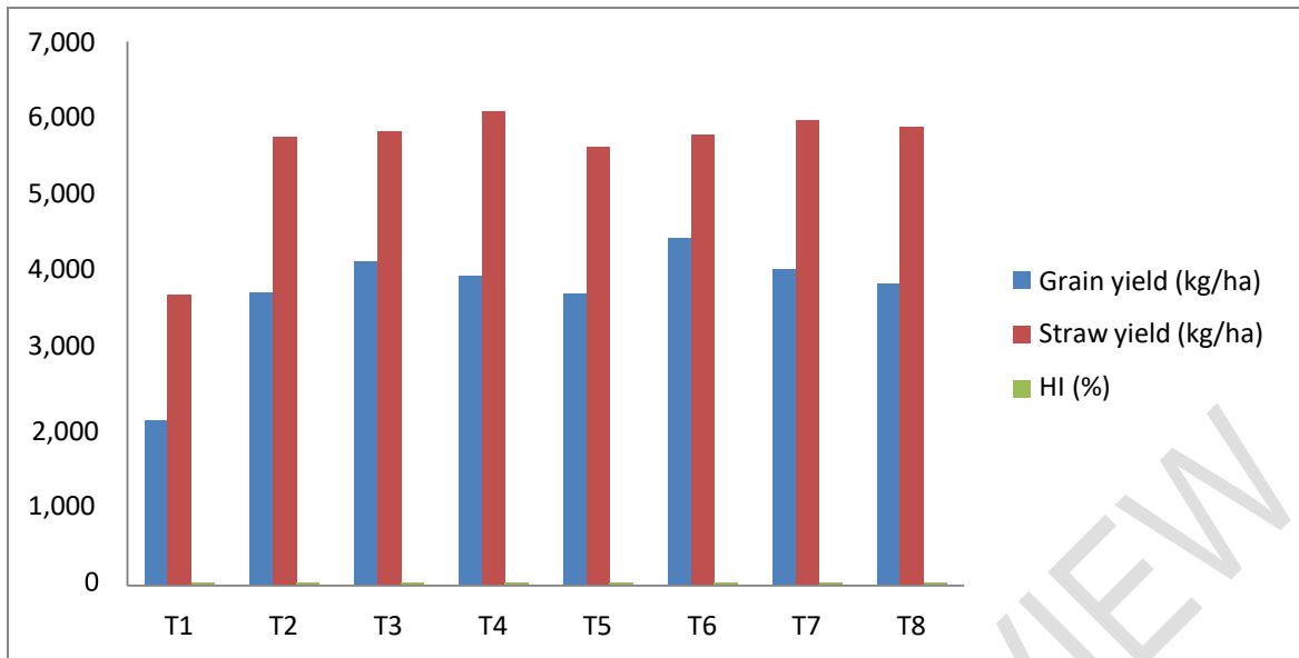
Fig. 1 Effect of integrated nutrient management on grain, straw yield ha -1 , harvest index of
