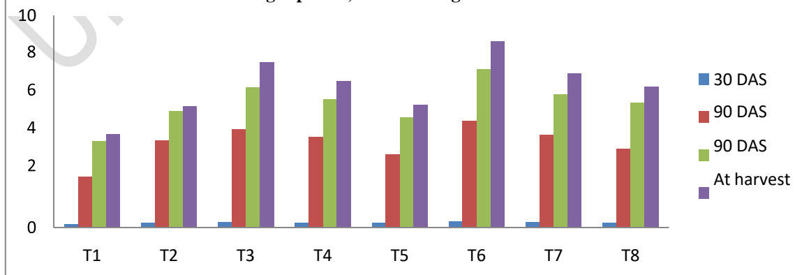
Fig.3 Effect of integrated nutrient management on dry matter accumulation (DMA) of wheat
