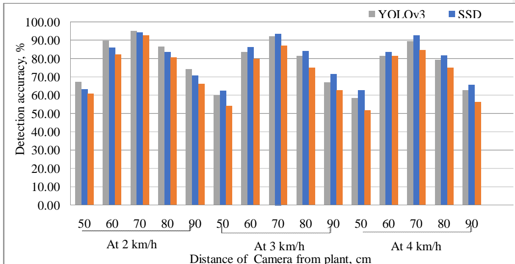
Figure 7. Dragon Fruit Size Detection Performance of Developed Yield Estimating System at Different Operating Speeds Using Different Deep Learning models.
