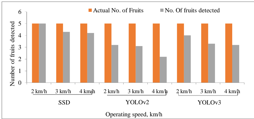
Fig. 6. Dragon fruit Detection Performance of Developed Yield Estimating System at Different Operating Speeds Using Different Deep Learning models
