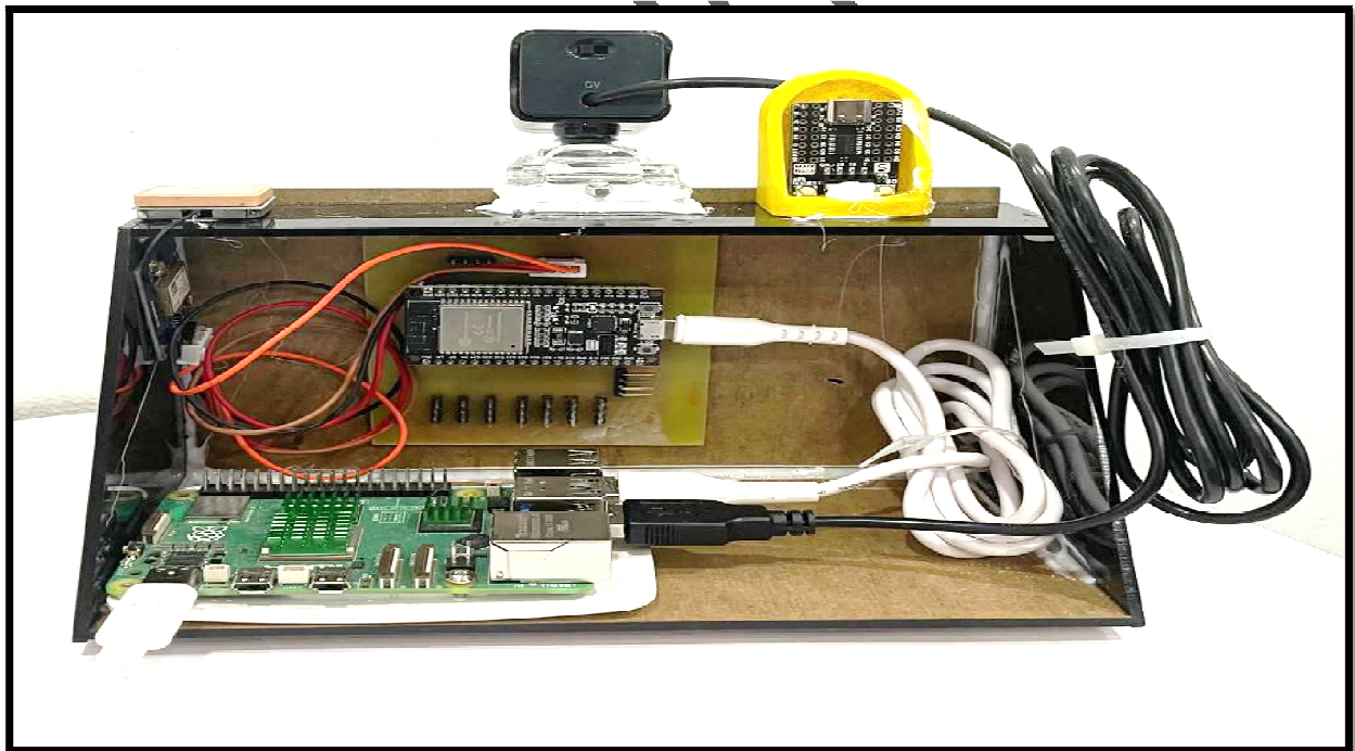
Fig 4. Completely assembled hardware of the system..
