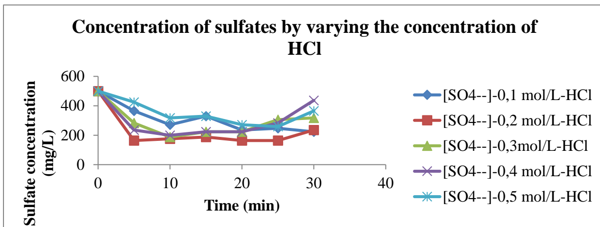
Figure 3: Concentration of sulfates as a function of time by varying the concentration of HCl, for a quantity of 3g CaCO 3 with initial sulfate concentration of 500mg/L.
