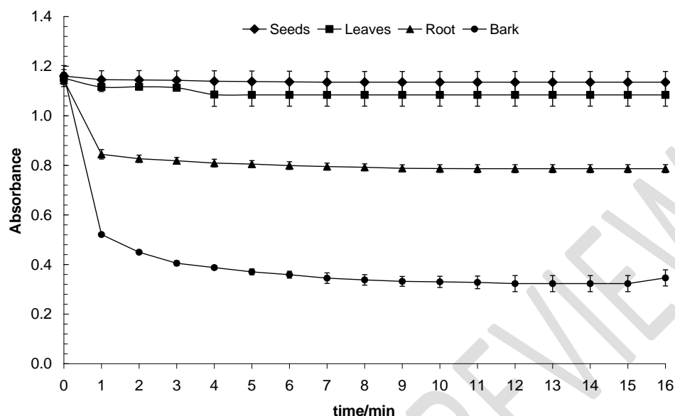
Figure 4. Decrease in absorbance of DPPH with A. pavonina Soxhlet extracts, over 16 minutes.
