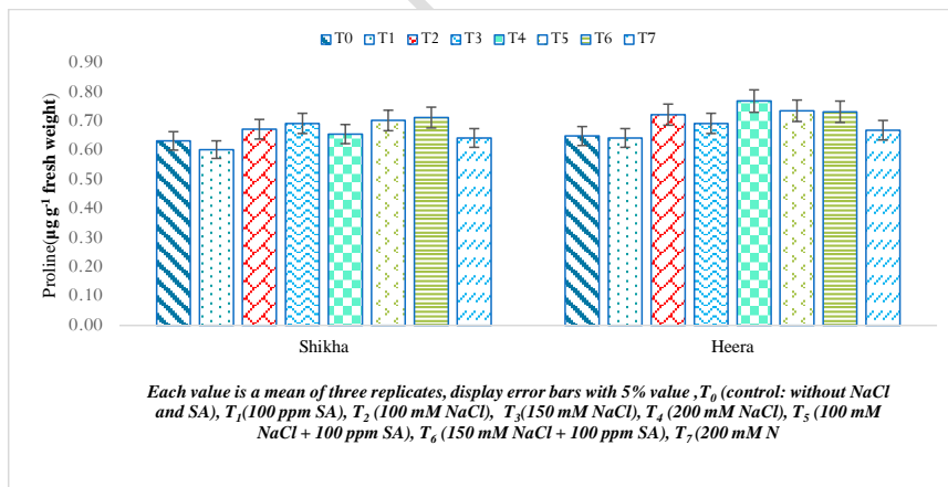
Fig 2: Influence of foliar spray of Salicylic acid (SA) on proline content ( \mu\text{g g}^{-1} fresh weight) in mungbean leaf under induced salt stress
