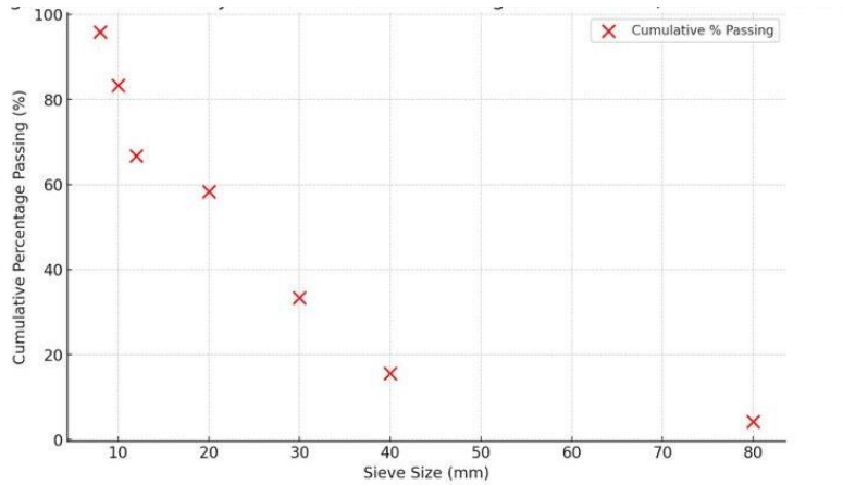
Figure 3: Sieve Analysis - Cumulative Percentage Passing vs Sieve Size (Scatter plot in Red)
