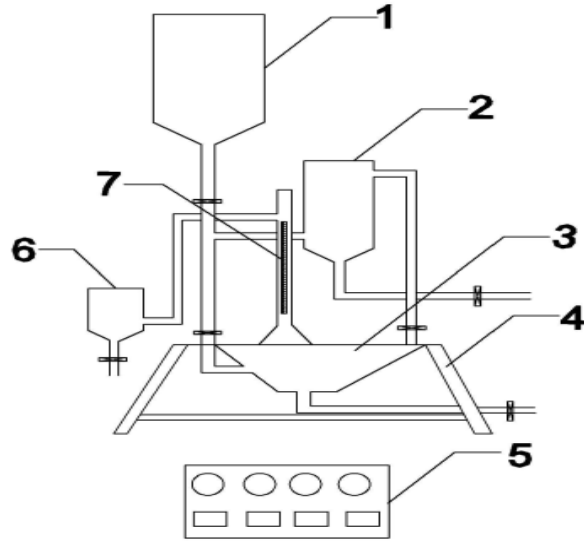
Figure 2: Line drawing of the clarifier unit that was developed
