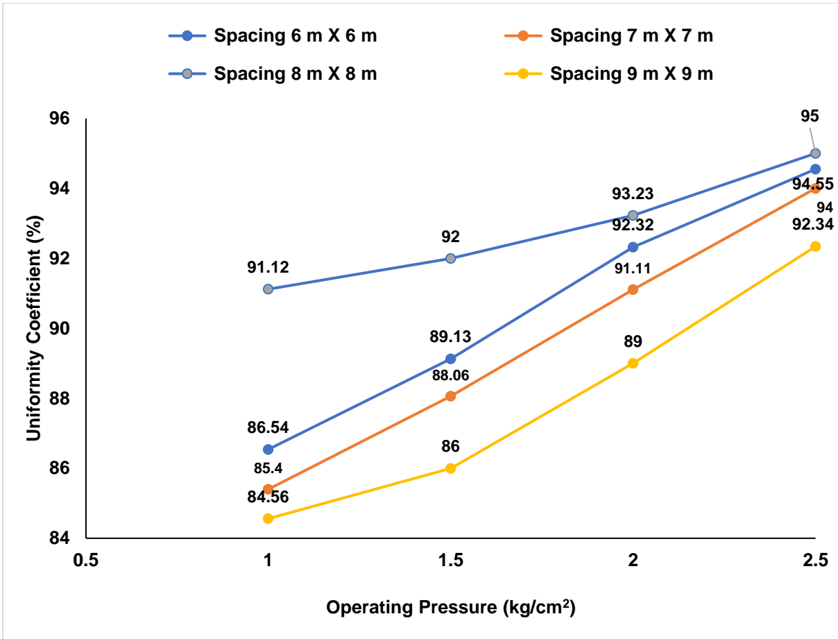
Fig. 3. Uniformity Coefficient at various operating pressures
