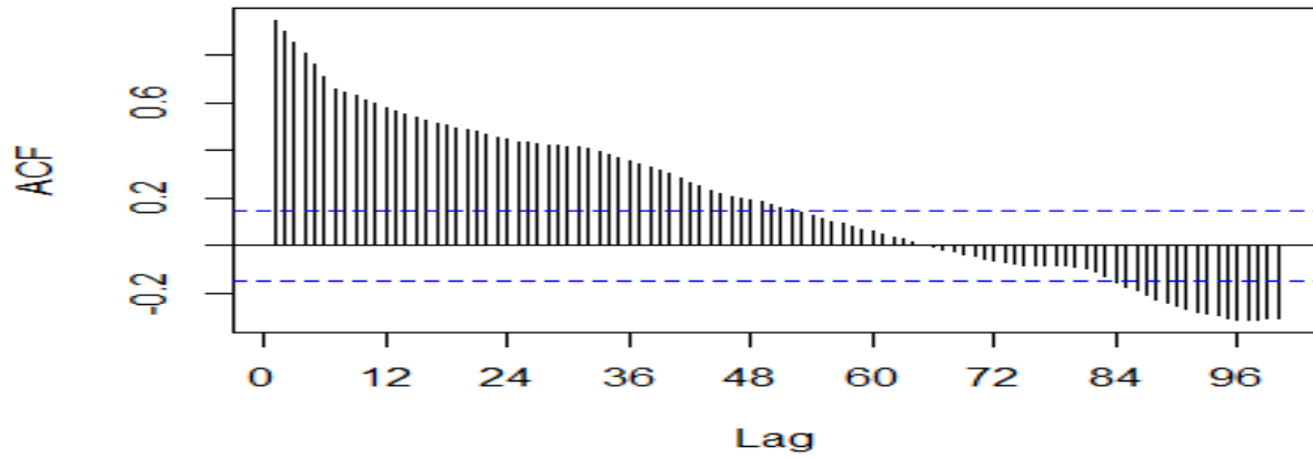
Fig 5- ACF of the trained data
