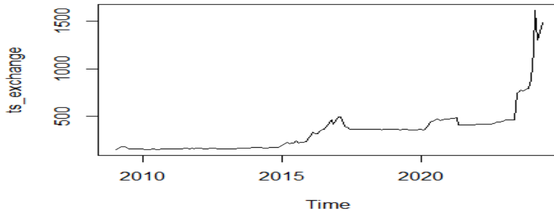
Fig 1: Time plot of Nigeria foreign exchange rate from January 2009 to May 2024 The time series plot of the Exchange Rate in Figure 1 exhibits trend indicating that the monthly exchange rate is changing over time. Especially from 2015 upward.
