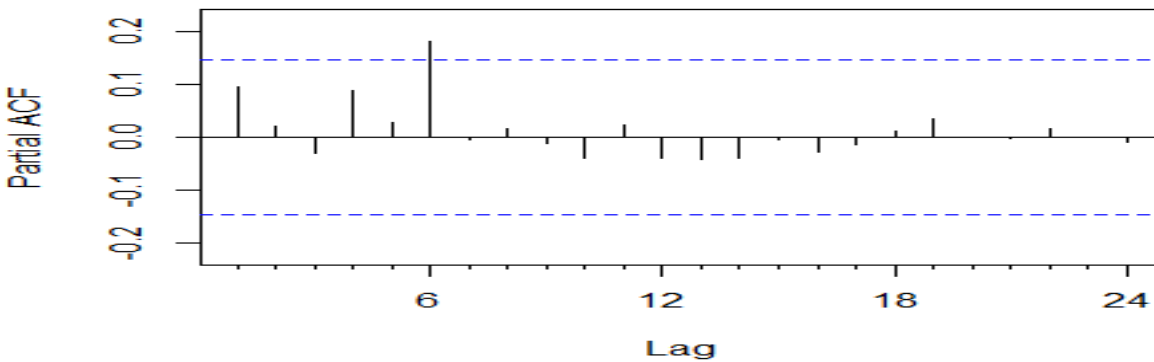
Figure 8, is the partial ACF of the rained data.
