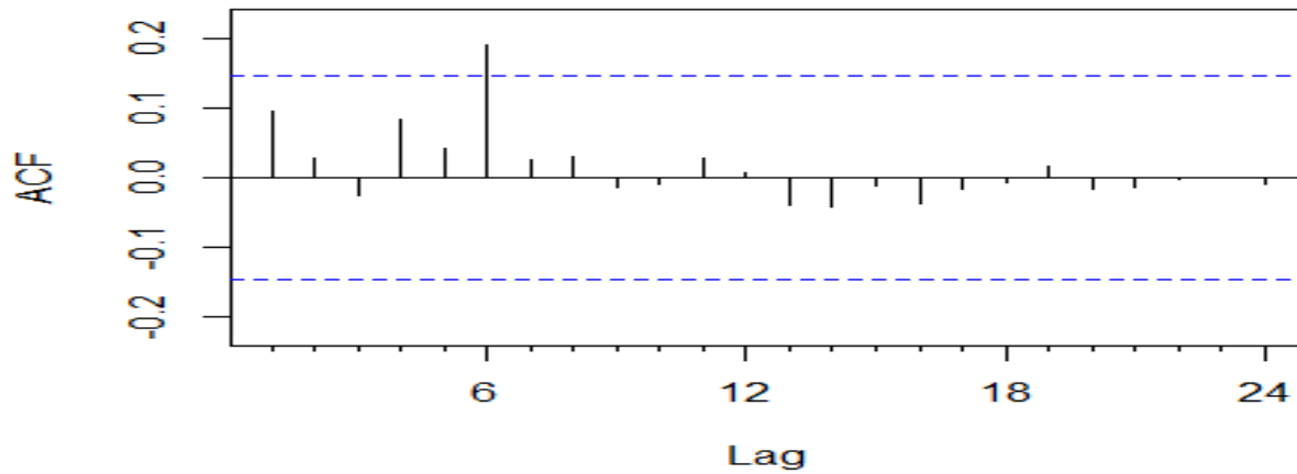
Fig 7- after the first difference the trained series
