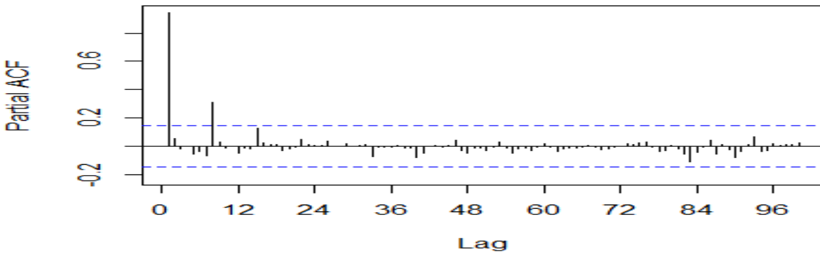
Figure 6, showing the partial ACF of the trained data
