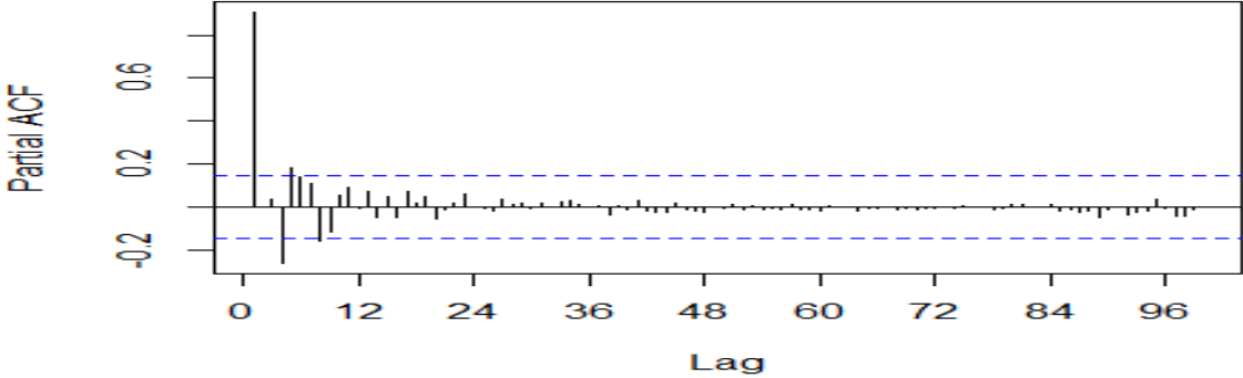
Figure 4, showing the partial ACF of the whole raw data
