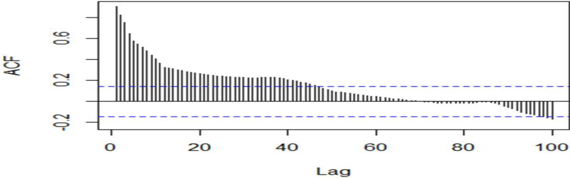
Fig 3- ACF of the whole raw data
