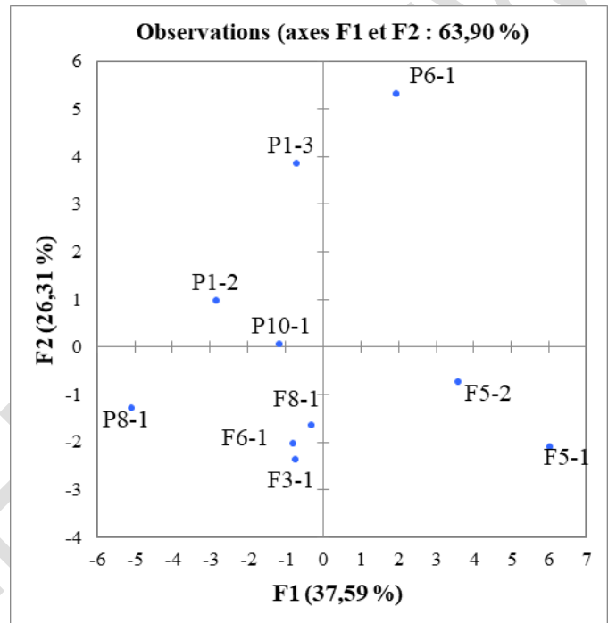
Fig. 5. Representation of wells and boreholes in the F1-F2 factorial plane
