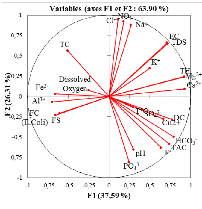
Fig. 4. Correlation circle
