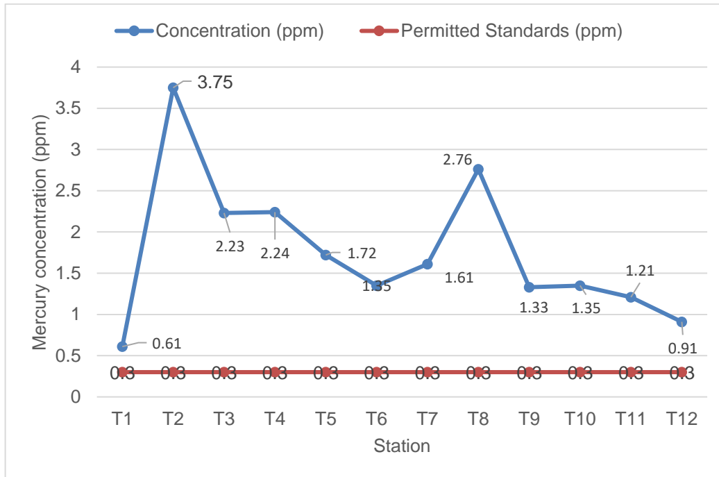
Figure 2. Mercury concentration in sediments of Taluduyunu River (Source: Laboratory Test Results, 2024)
