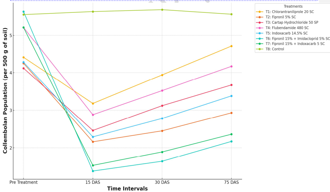
Fig 2. Effect of insecticides on collembolean population at different intervals
