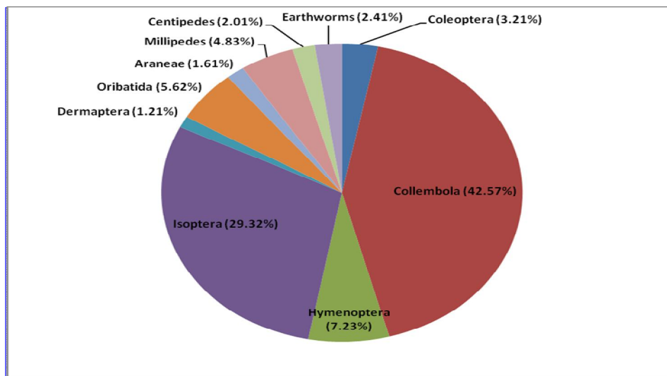
Fig 1. Relative Abundance of soil arthropods found in the experimental location
