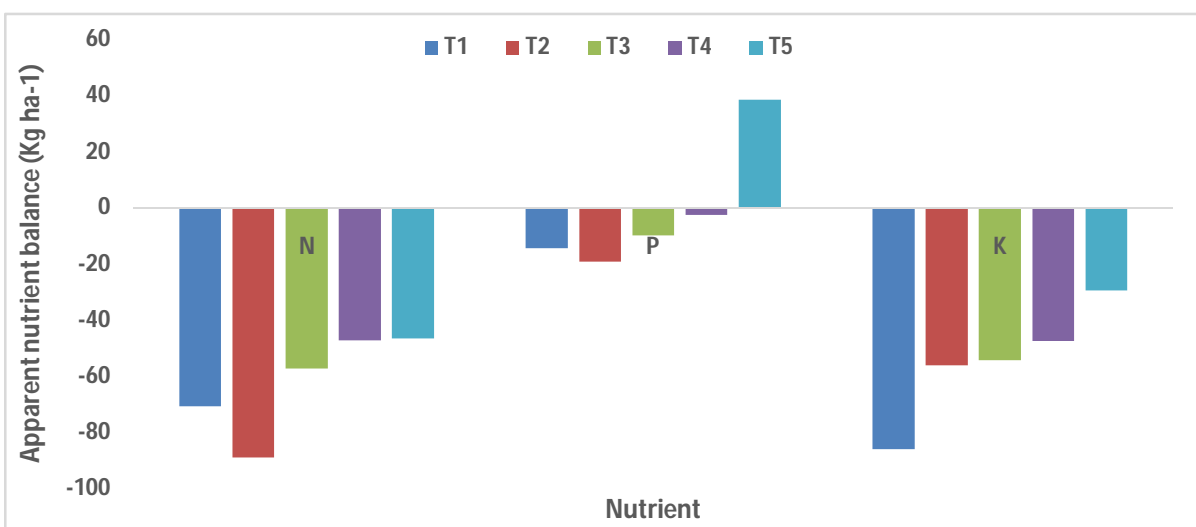
Figure 1: Effect of nutrient management practices on apparent nutrient balance of rice-rice cropping system
